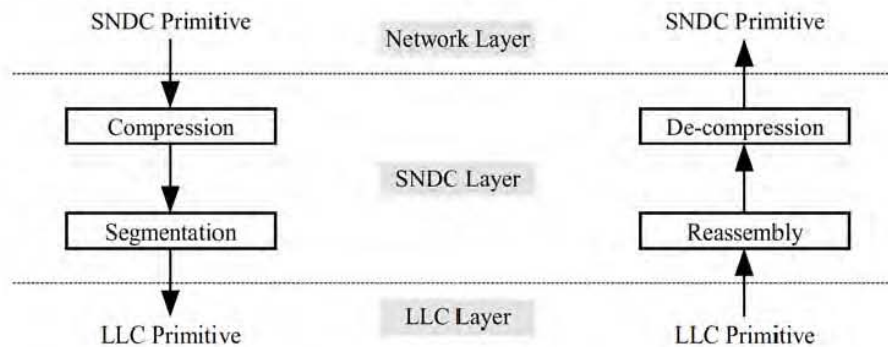
Figure 47: Sequential Invocation of SNDC Functionality
