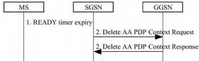
Figure 44: Anonymous Access PDP Context Deactivation Initiated by MS Procedure
