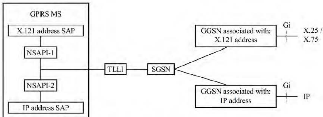
Figure 51: Use of NSAPI and TLLI
