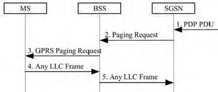
Figure 33: GPRS Paging Procedure
