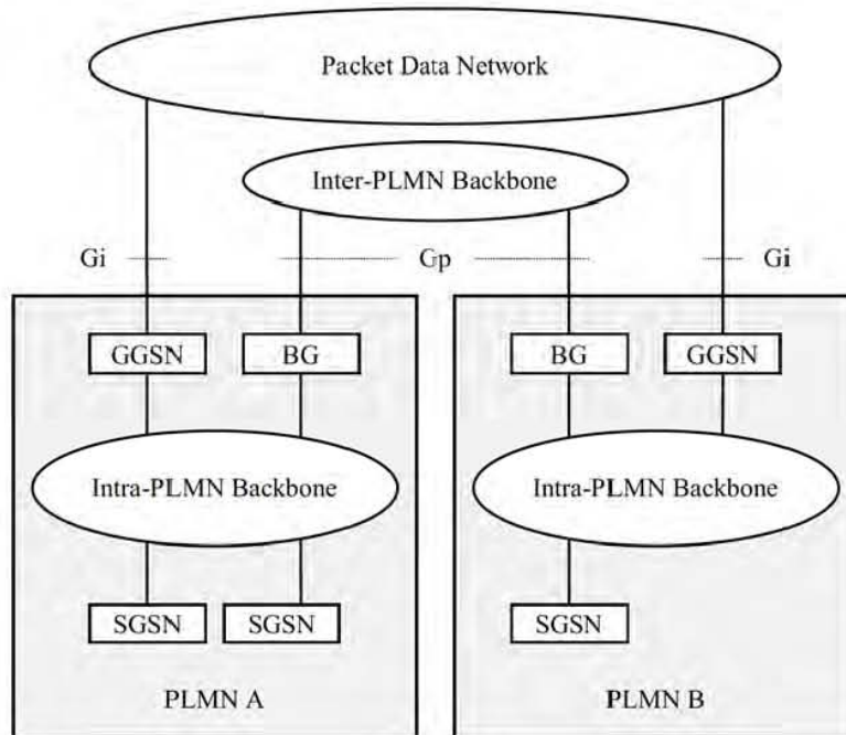
Figure 3: Intra- and Inter-PLMN Backbone Networks
