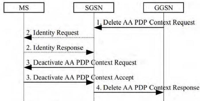
Figure 45: Anonymous Access PDP Context Deactivation Initiated by GGSN Procedure
