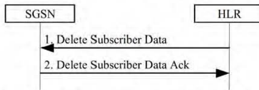
Figure 32: Delete Subscriber Data Procedure
