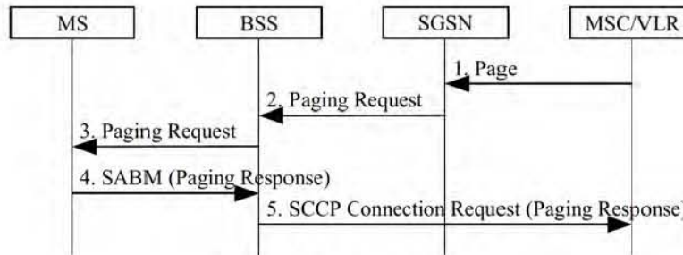
Figure 15: CS Paging Procedure
