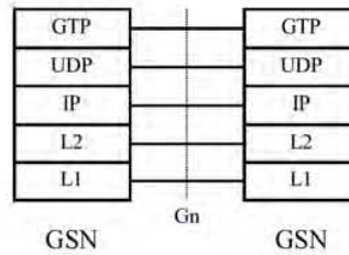
Figure 10: Signalling Plane GSN - GSN
