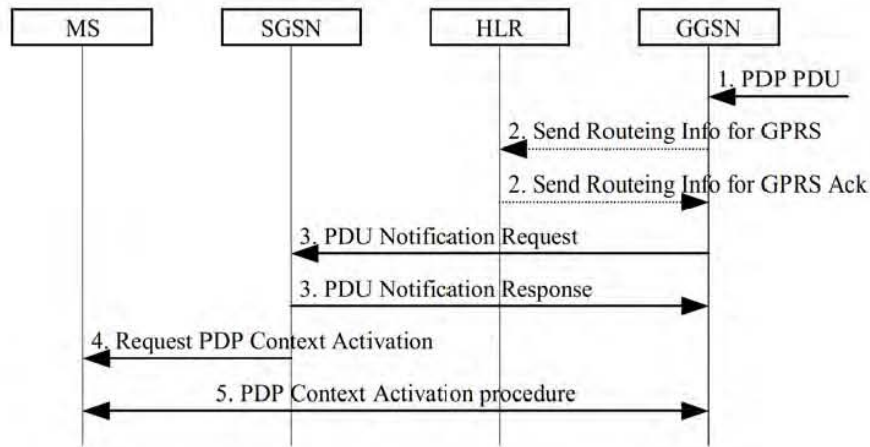
Figure 36: Successful Network-Requested PDP Context Activation Procedure
