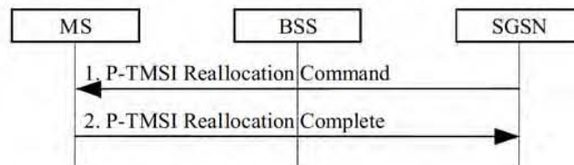
Figure 24: P-TMSI Reallocation Procedure
