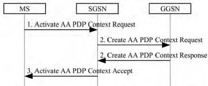
Figure 39: Anonymous Access PDP Context Activation Procedure
