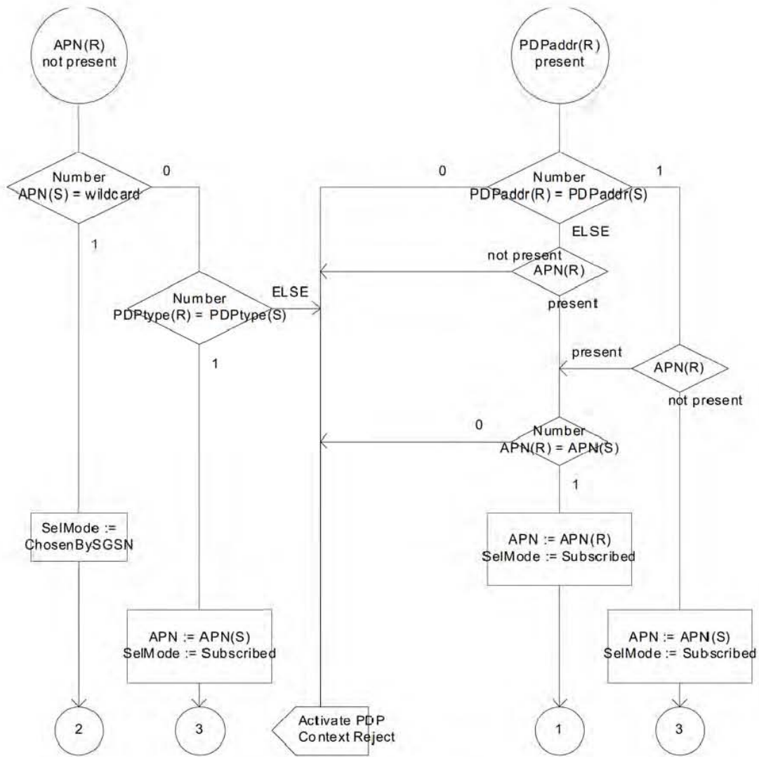
Figure A.3: SDL Diagram 3
