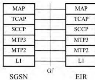
Figure 8: Signalling Plane SGSN - EIR
