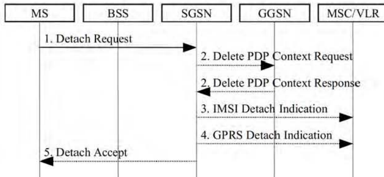
Figure 19: MS-Initiated Combined GPRS / IMSI Detach Procedure
