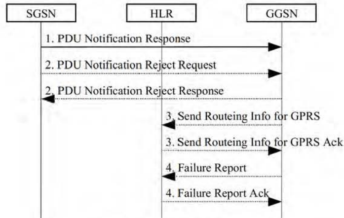
Figure 37: Protection Procedure
