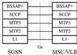
Figure 7: Signalling Plane SGSN - MSC/VLR
