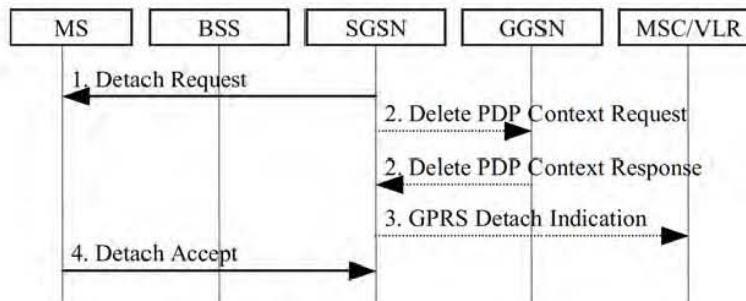
Figure 20: SGSN-Initiated GPRS Detach Procedure
