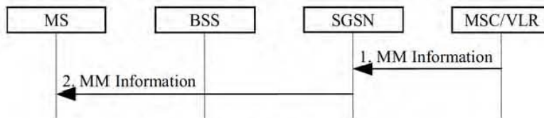
Figure 17: MM Information Procedure
