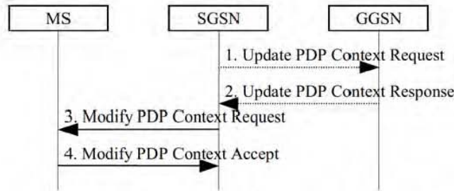
Figure 40: PDP Context Modification Procedure
