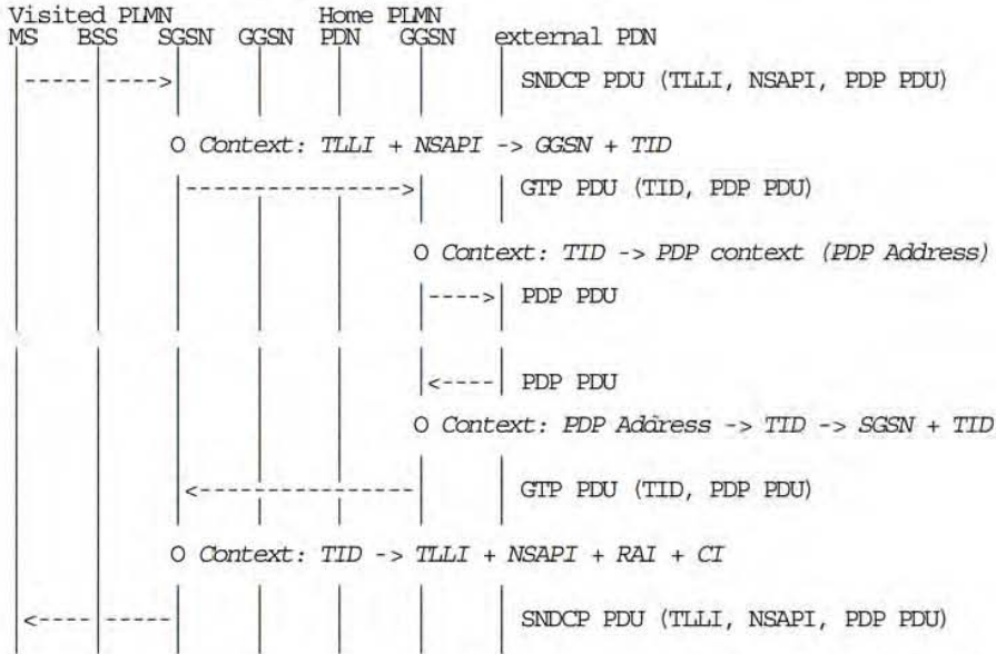
Figure B.2: Data Routing for a Roaming MS to and from an External PDN
