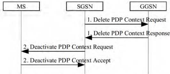
Figure 42: PDP Context Deactivation Initiated by SGSN Procedure
