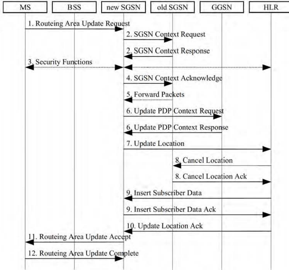
Figure 28: Inter SGSN Routing Area Update Procedure
