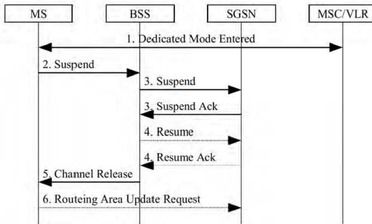
Figure 55: Suspend and Resume Procedure
