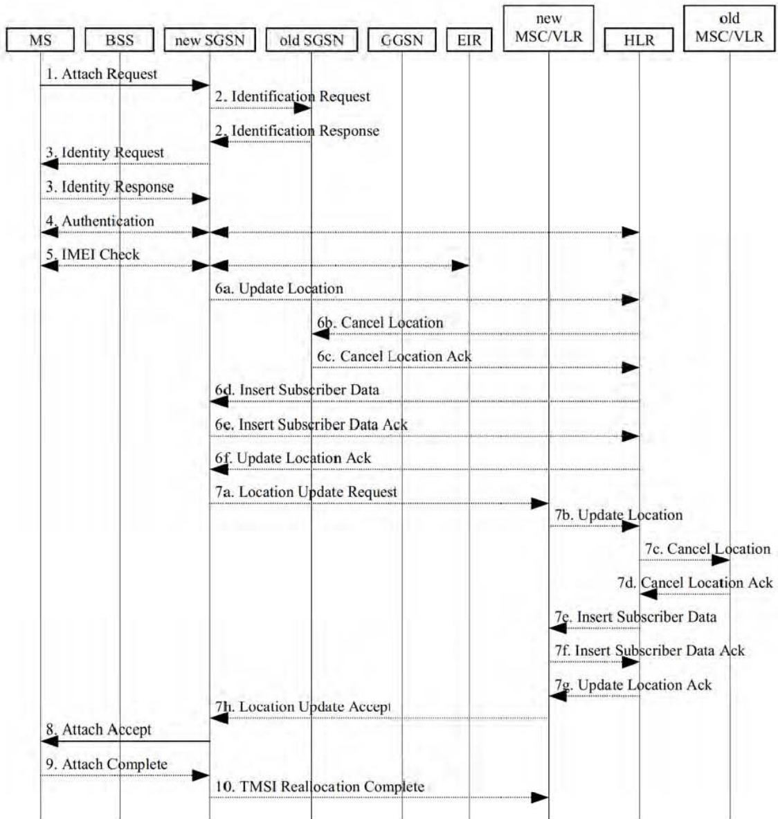
Figure 18: Combined GPRS / IMSI Attach Procedure
