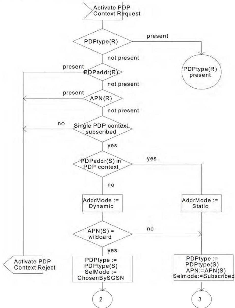
Figure A.1: SDL Diagram 1
