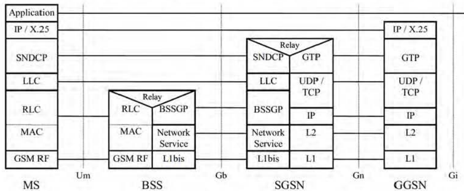
Figure 4: Transmission Plane
