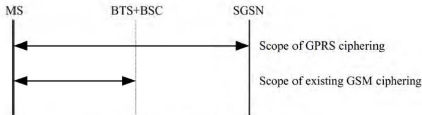
Figure 25: Scope of GPRS Ciphering
