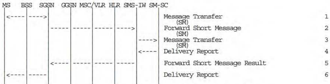
Figure 54: MO SMS Transfer, Successful
