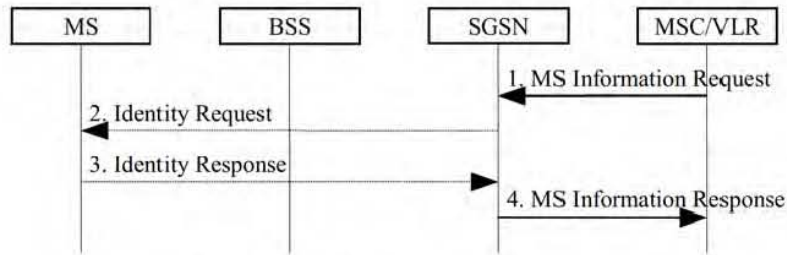
Figure 16: MS Information Procedure
