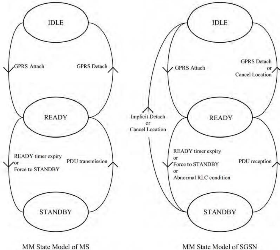
Figure 13: Functional Mobility Management State Model
