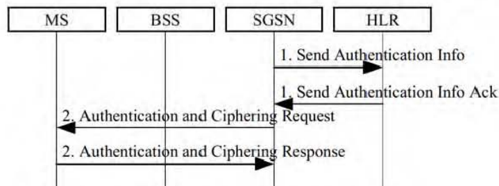
Figure 23: Authentication Procedure
