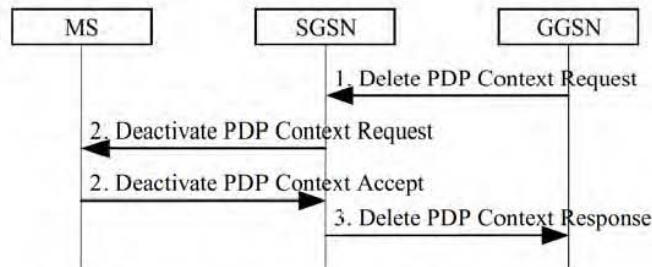
Figure 43: PDP Context Deactivation Initiated by GGSN Procedure
