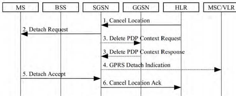
Figure 21: HLR-Initiated GPRS Detach Procedure
