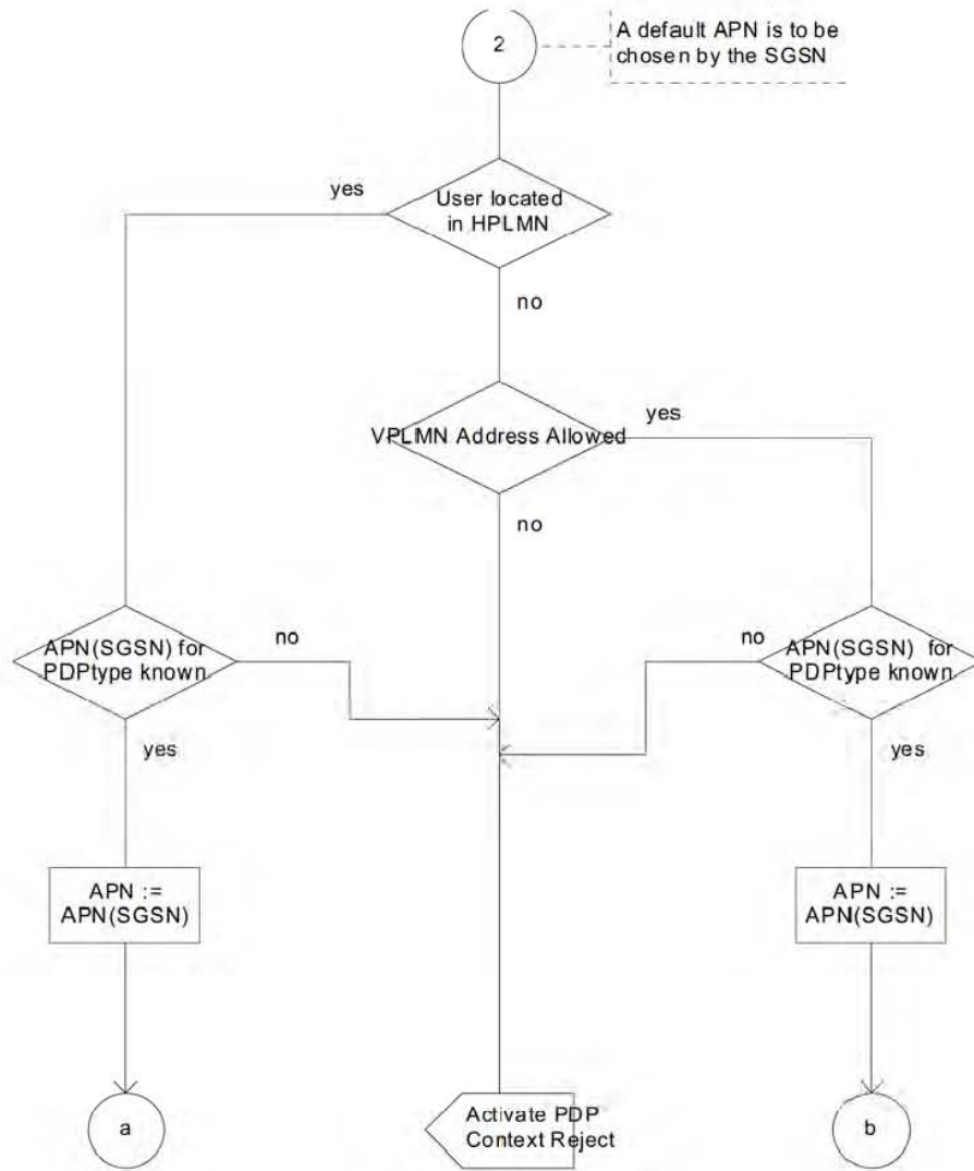
Figure A.5: SDL Diagram 5
