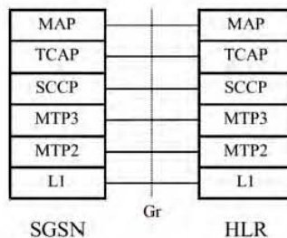
Figure 6: Signalling Plane SGSN - HLR
