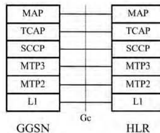
Figure 11: Signalling Plane GGSN - HLR Using MAP
