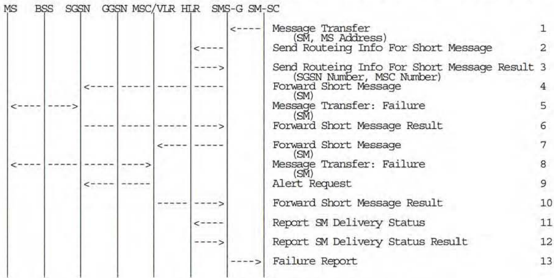
Figure 53: MT SMS Transfer, Unsuccessful
