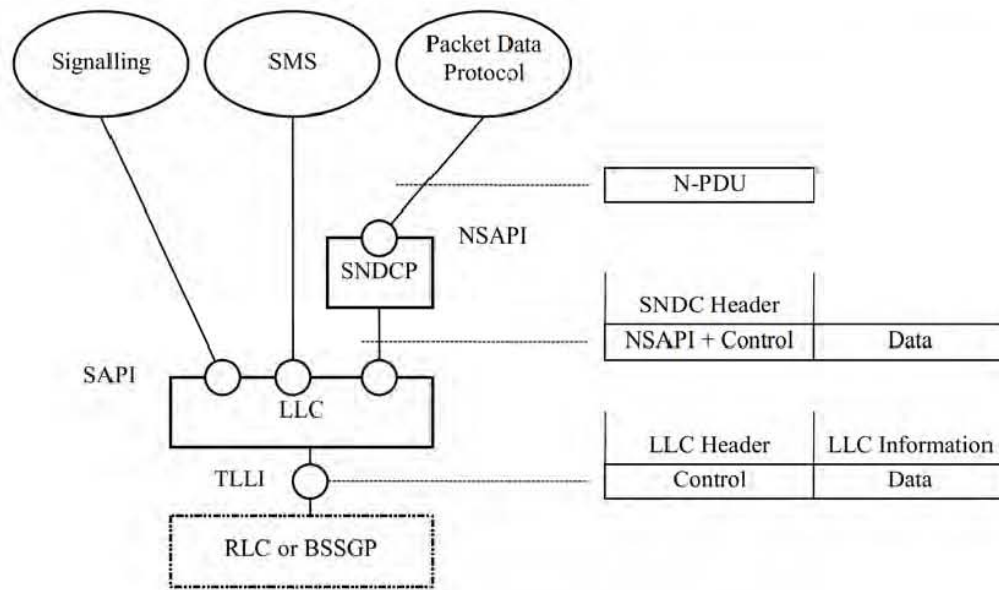
Figure 46: Multiplexing of Network Protocols
