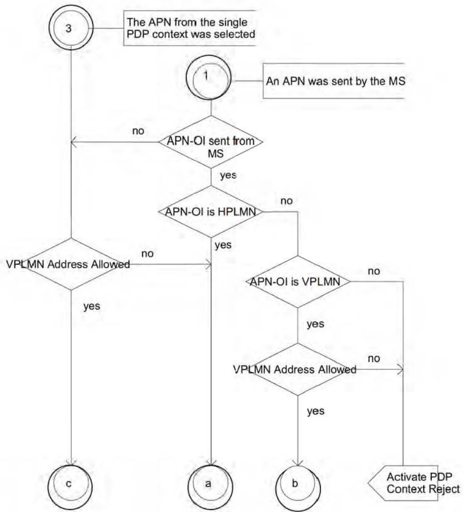
Figure A.4: SDL Diagram 4
