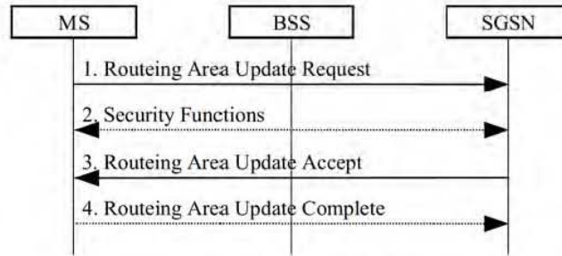
Figure 27: Intra SGSN Routing Area Update Procedure
