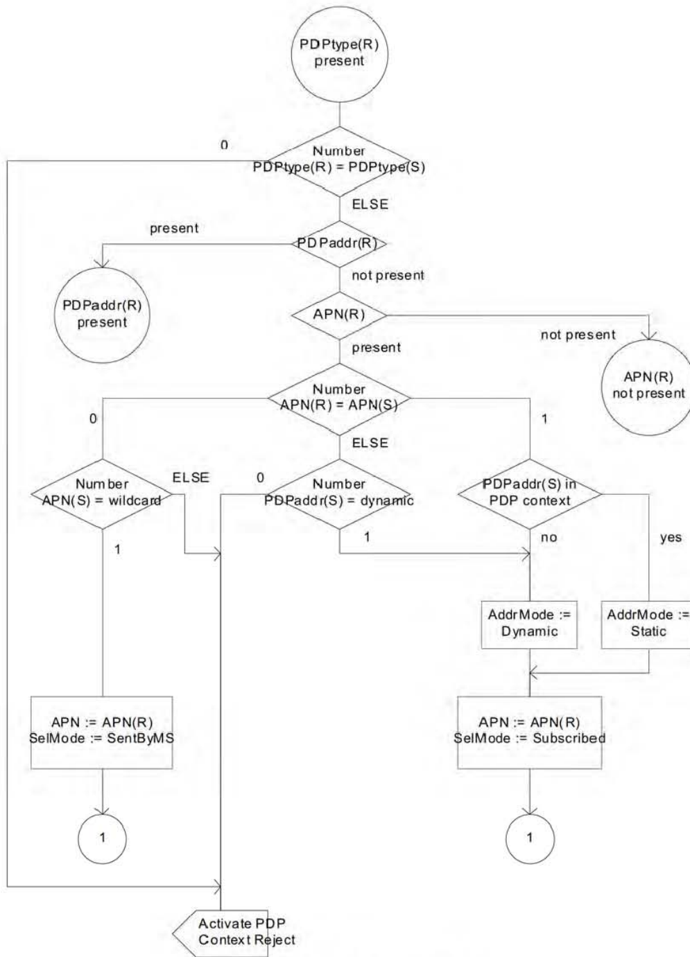
Figure A.2: SDL Diagram 2
