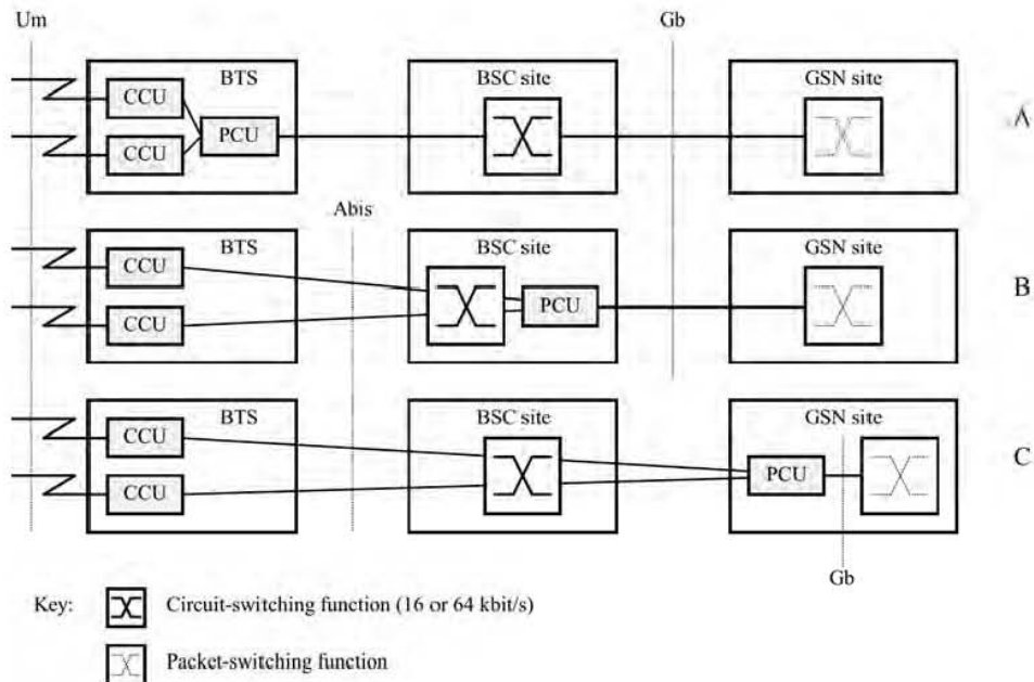
Figure 49: Remote Packet Control Unit (PCU) Positions
