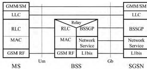
Figure 5: Signalling Plane MS - SGSN
