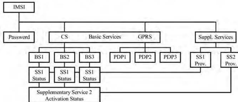
Figure 50: GPRS Subscription Data
