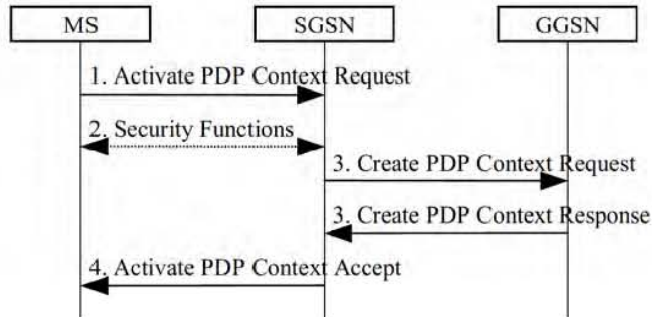
Figure 35: PDP Context Activation Procedure
