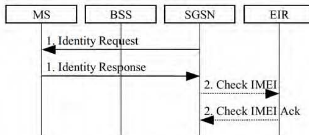
Figure 26: Identity Check Procedure
