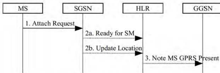
Figure 38: Mobile User Activity Procedure
