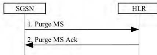
Figure 22: Purge Procedure
