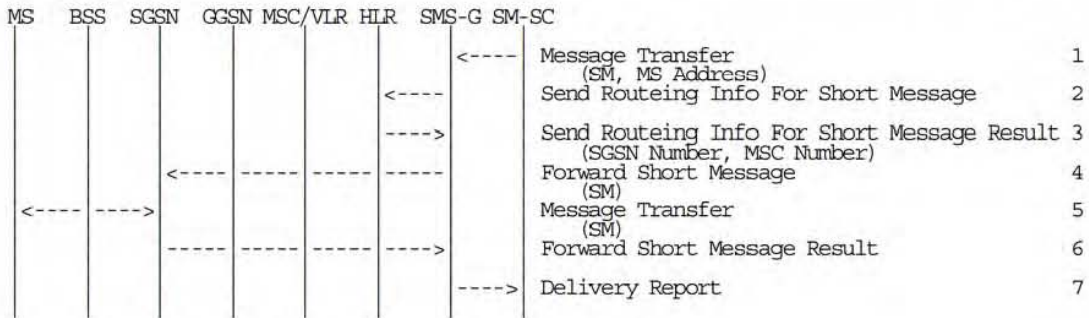
Figure 52: MT SMS Transfer, Successful
