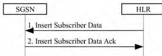
Figure 31: Insert Subscriber Data Procedure
