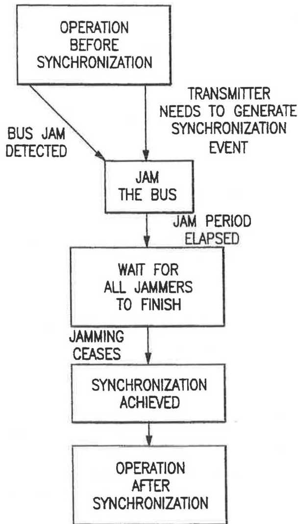
FSD FOR SYNCHRONIZATION OF MULTIPLE TRANSMITTERS.
