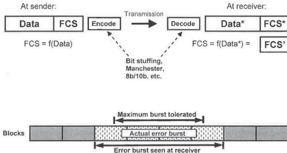
Figure A-2. Error Burst Length Extension Due to Encoding
