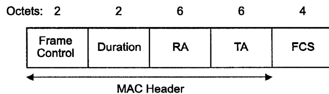
Figure 16—RTS frame
