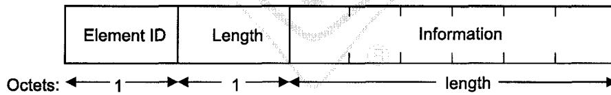
Figure 34—Element format
