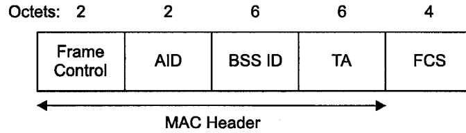
Figure 19—PS-Poll frame
