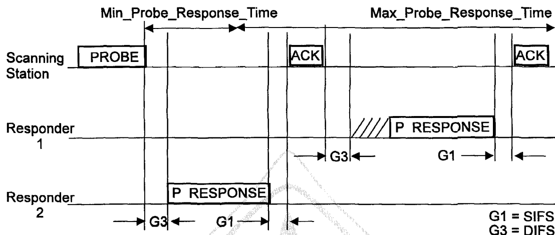
Figure 66—Probe response
