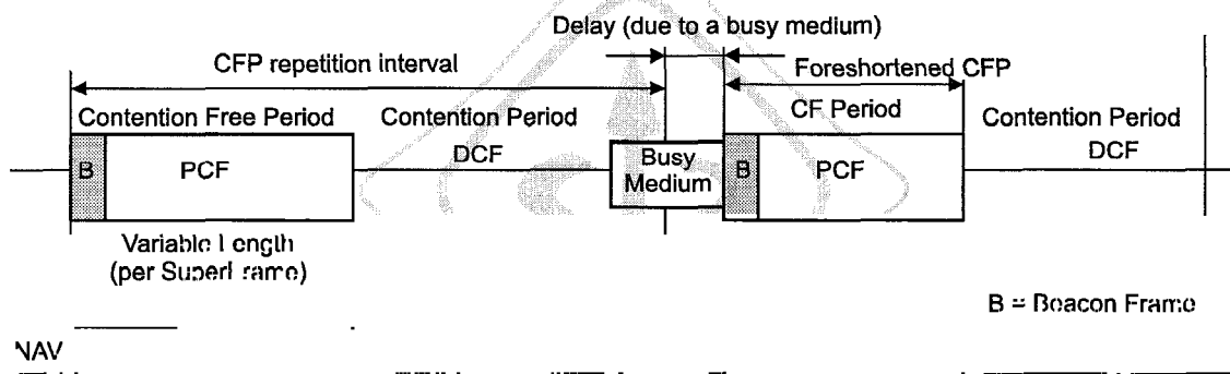
Figure 59—CFP/CP alternation
