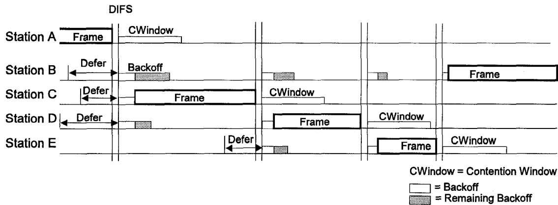
Figure 52—Backoff procedure
