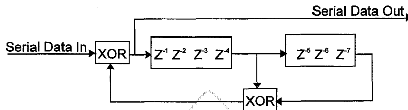
Figure 89—Data scrambler
