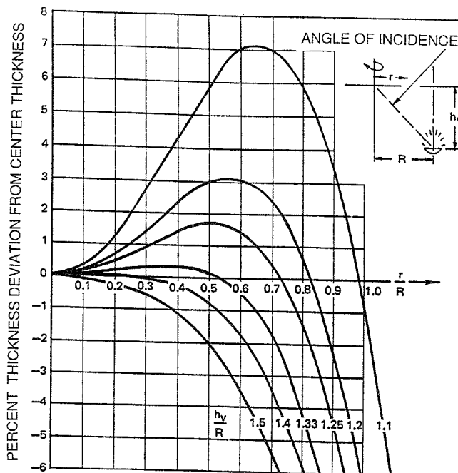
Figure 3-7. Calculated film thickness variation across the radius of a rotating disk. (From Ref. 10).
