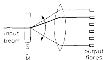
SLM acts as diffraction grating with a digitally tuneable grating period.
