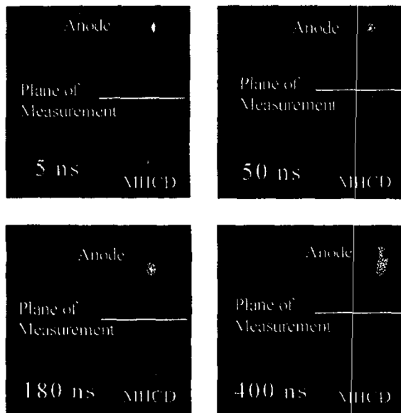
Figure 6. Photographs of the MCSG for different times after pulse application. Electrode gap: 2mm, applied electrical field: 10 kV/cm [6].
