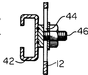
Fig. 2 PRIOR ART
