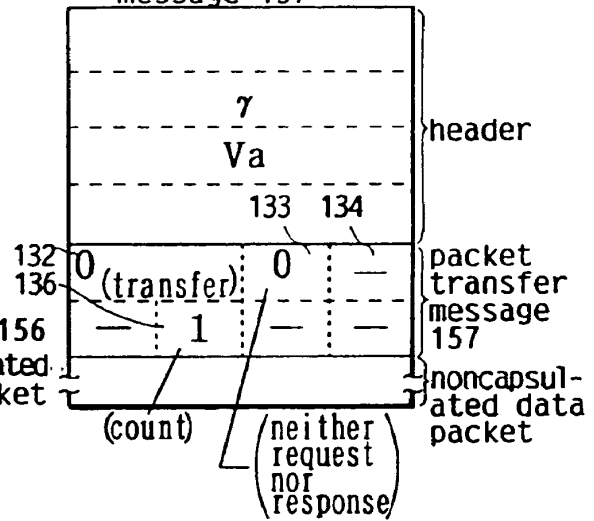
(2) data packet including message 157
