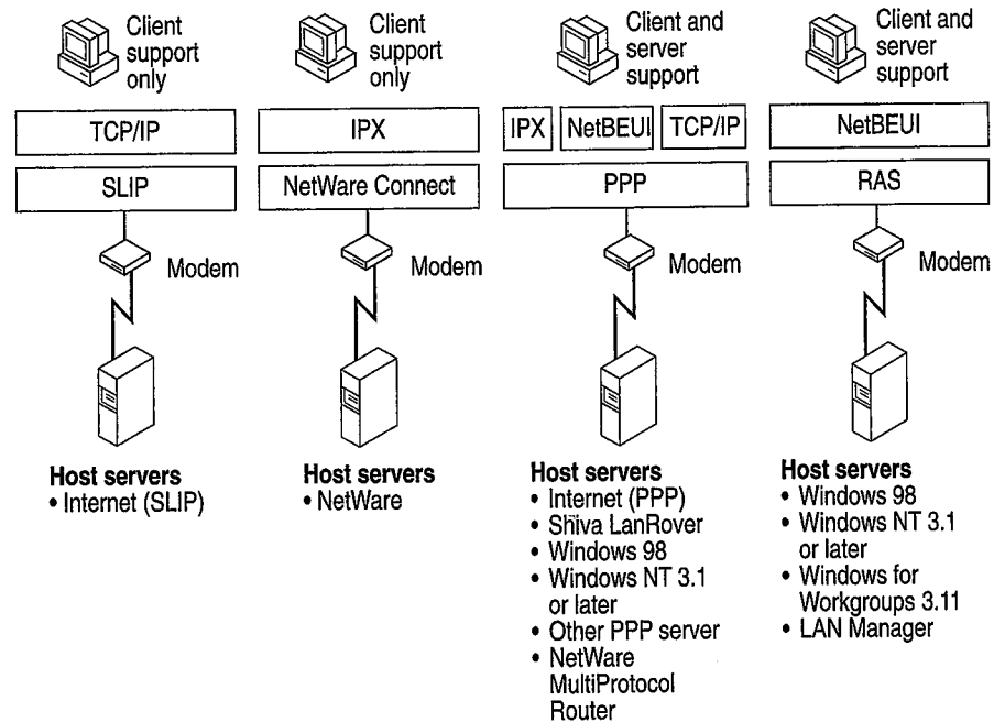
Figure 19.3 Connection protocols
