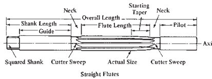
Hand Reamer, Pilot and Guide
