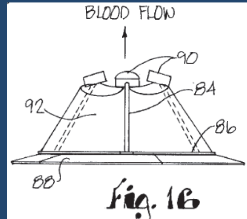
Trihedral Valve (5:33-62)
