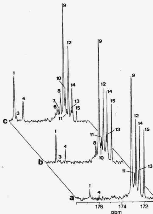
FIG. 1. Expansion of the carbonyl regions of the ^{13}\text{C} nuclear magnetic resonance spectra of lipids extracted from raw (a), cooked (b) and canned (c) tuna muscles. Labeled peaks are assigned as shown in Table 1.
