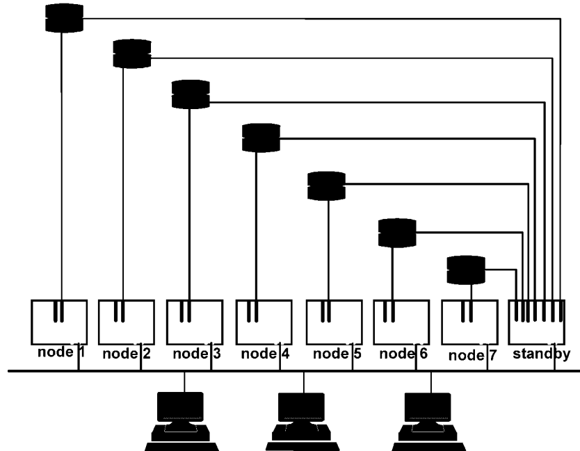
Eight-Node Active/Standby Cluster
