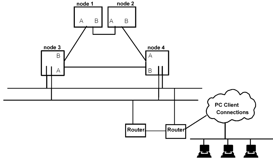
Figure 2-3 Configuration with Dual Attach FDDI Stations
