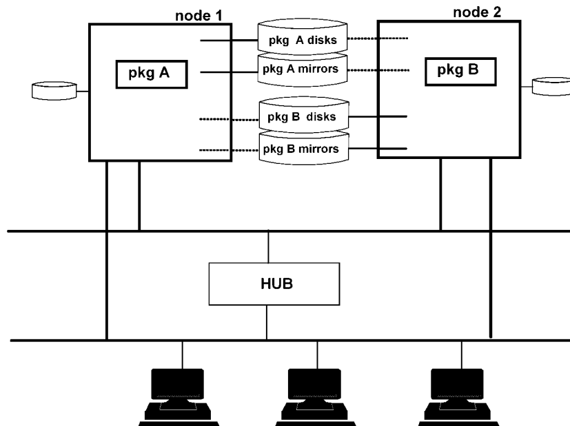
Typical Cluster Configuration
