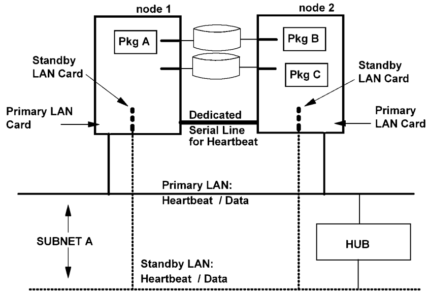
Figure 2-5 Serial (RS232) Heartbeat Line
