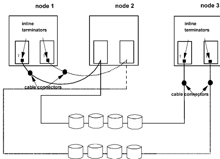
Figure 8-1 F/W SCSI Buses with In-line Terminators
