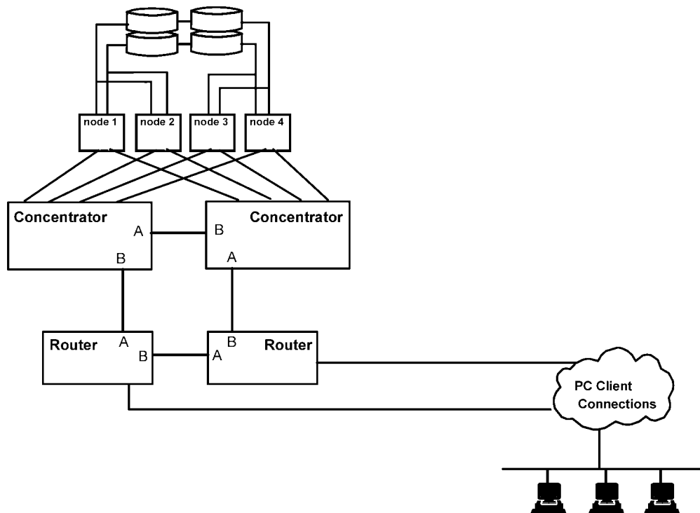
Figure 2-2 Redundant FDDI Configuration
