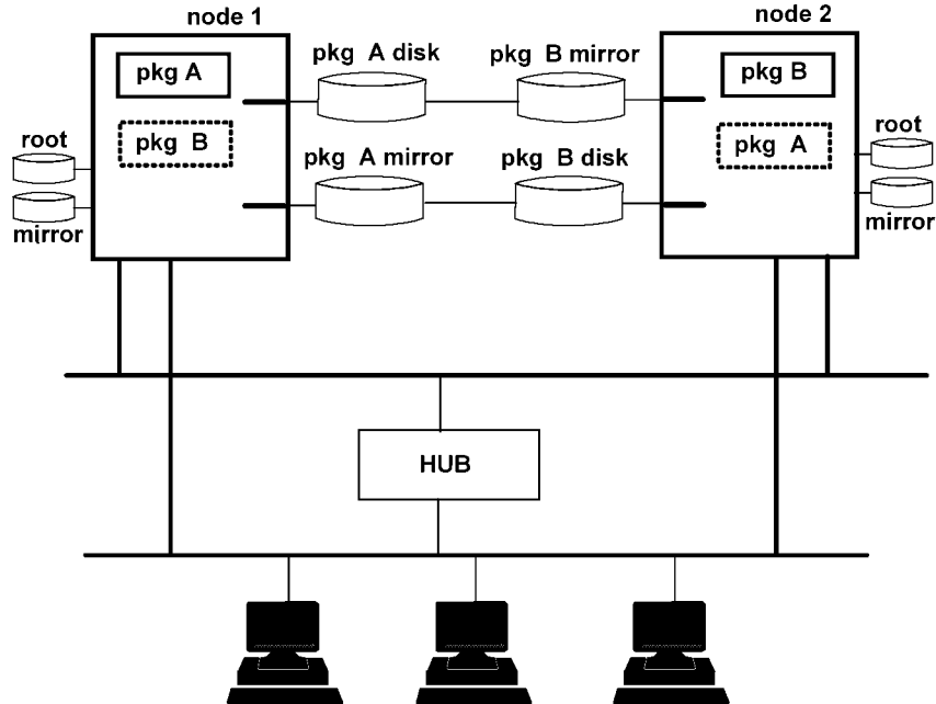
Figure 2-6 Mirrored Disks Connected for High Availability
