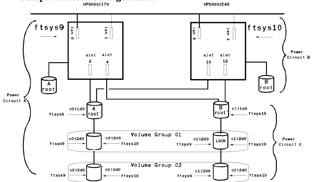
Figure 4-1 Sample Cluster Configuration
