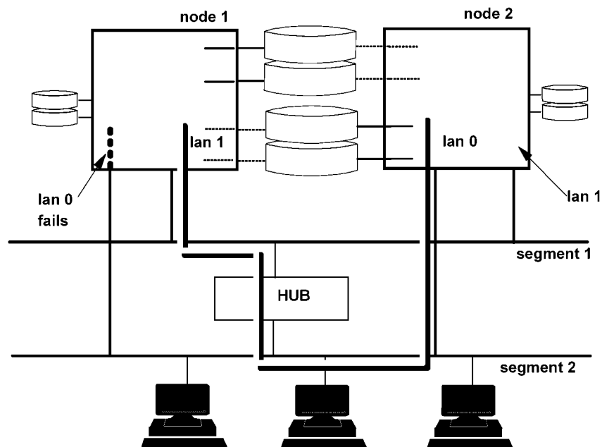
Figure 3-3 Cluster After Local Network Switching
