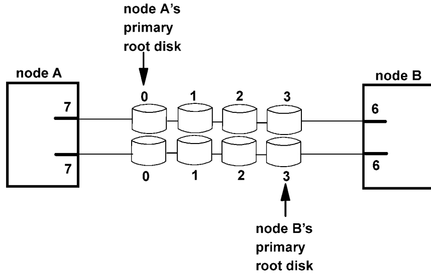
Figure 2-8 Root Disks on Different Shared Buses
