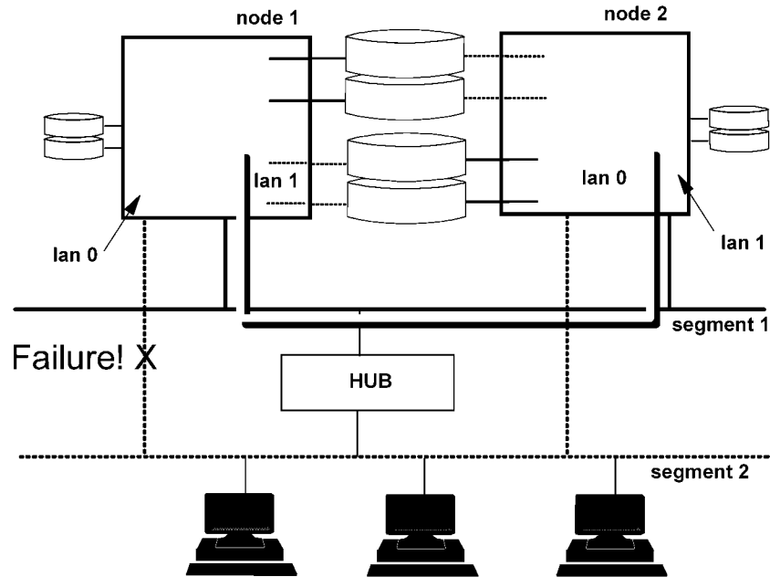
Figure 3-4 Local Switching After Cable Failure
