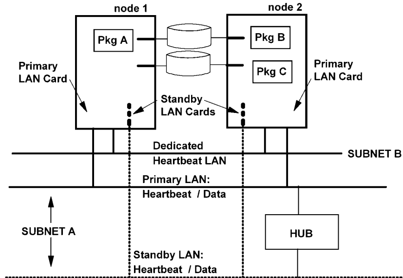
Figure 2-1 Redundant LANs
