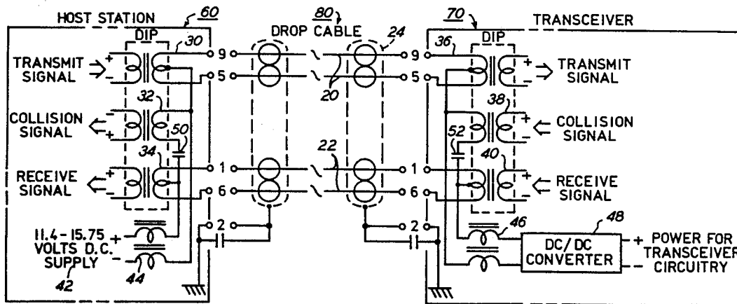
PROPOSED AND DEMONSTRATED ETHERNET DROP CABLE CONCEPT
