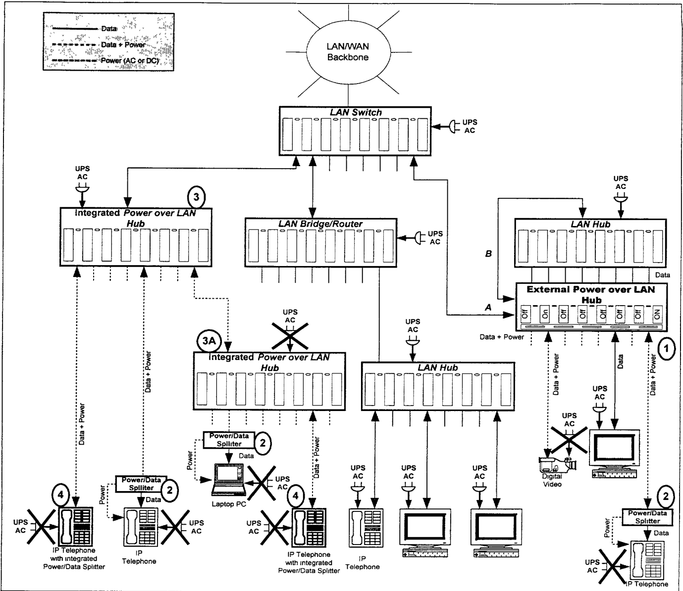
Figure 1 – Power over LAN Typical network installation
