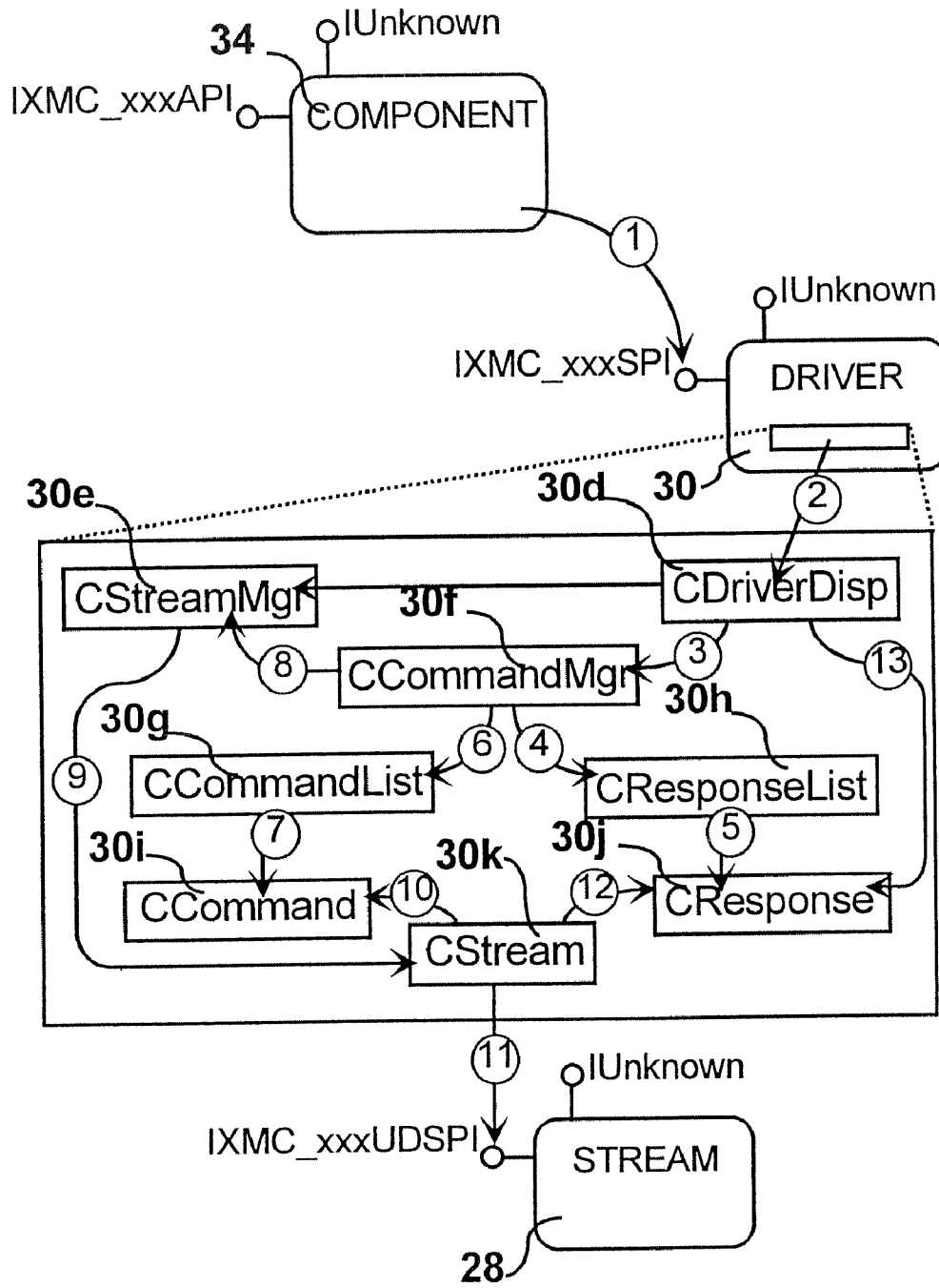
FIG. 19 Scenario-Map - Command Operations
