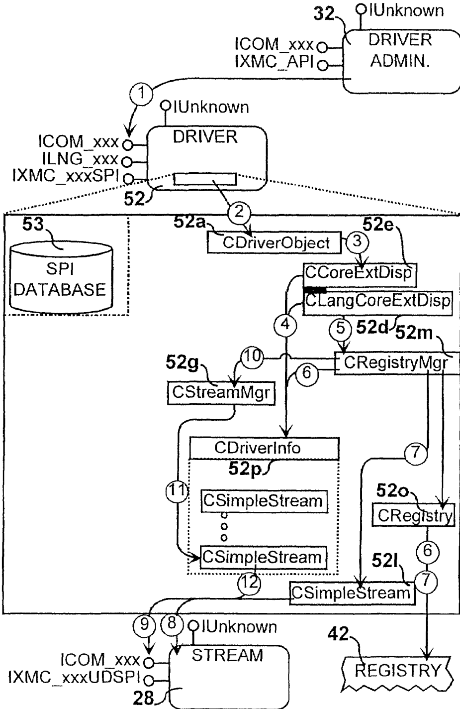
FIG. 63 Scenario-Map - Registration loading
