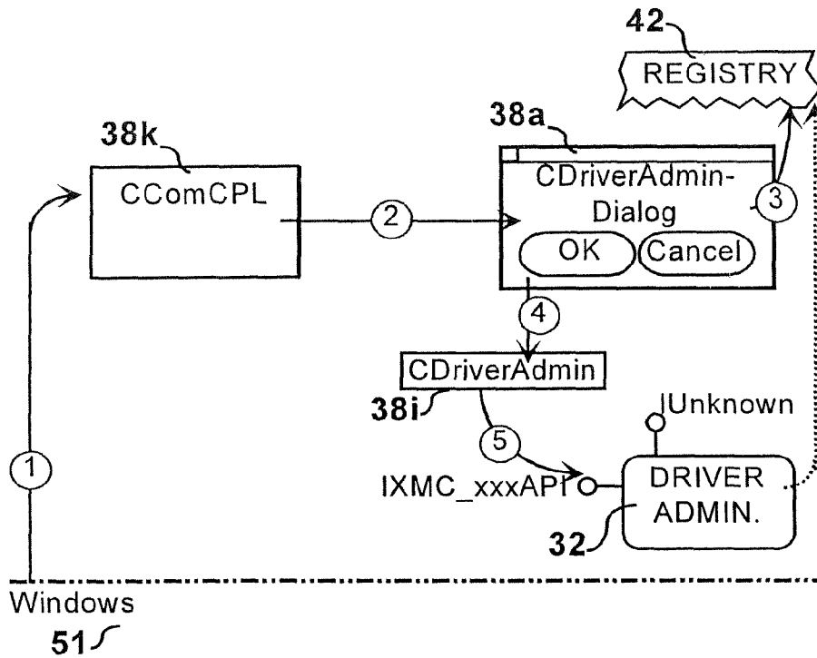
FIG. 53 Scenario-Map - Initializing the App.
