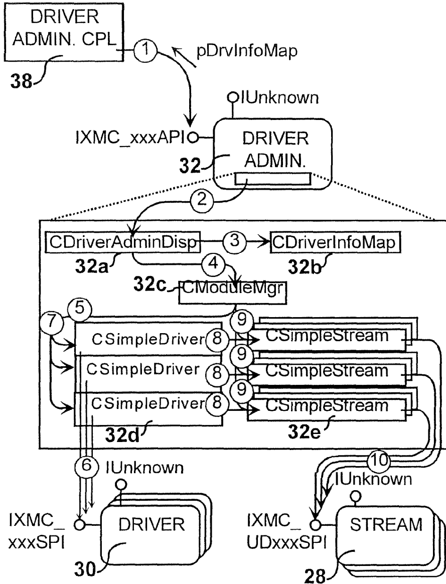
FIG. 48 Scenario-Map - Querying Drv Info. Map
