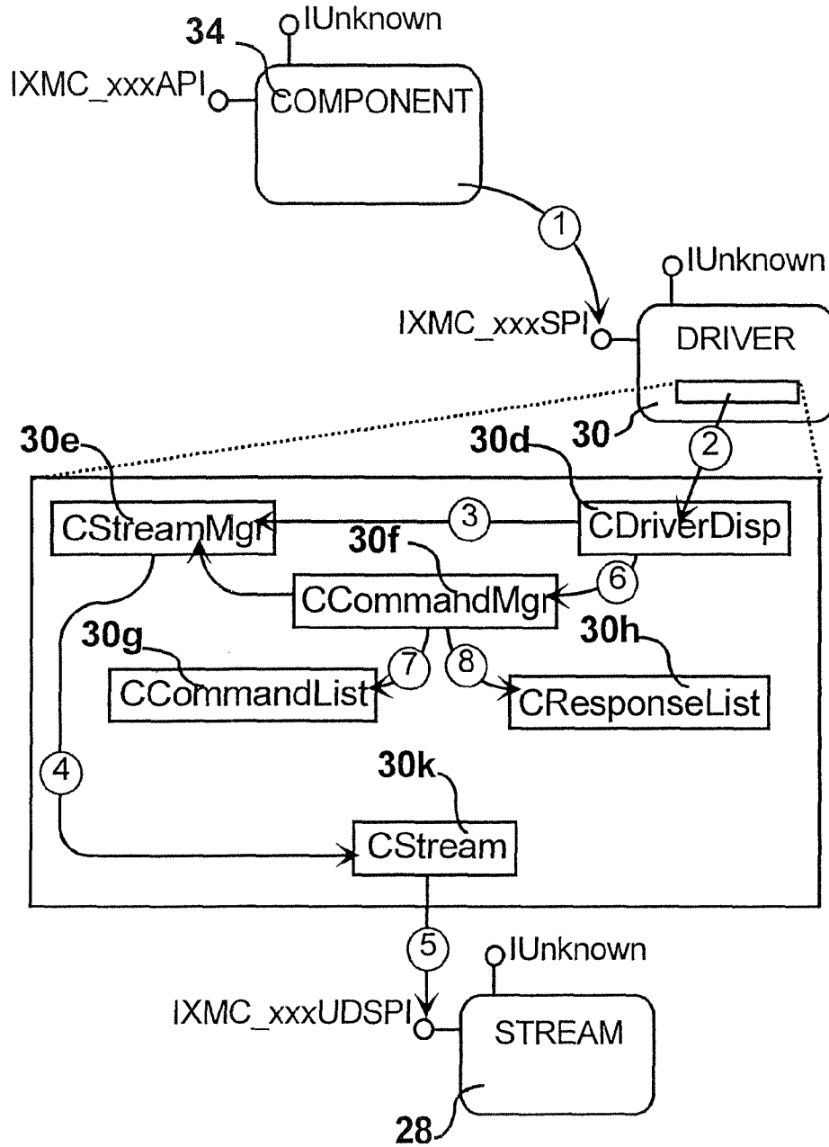
FIG. 20 Scenario-Map - Clean-up by Component
