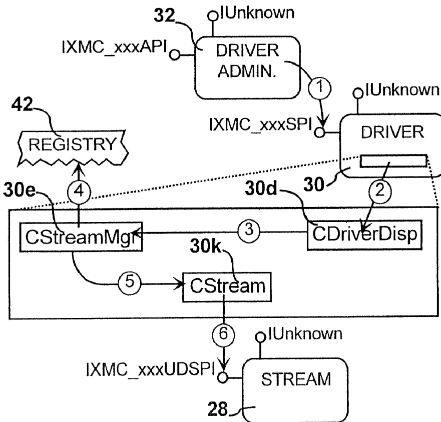
FIG. 16 Scenario-Map - Query Operation
