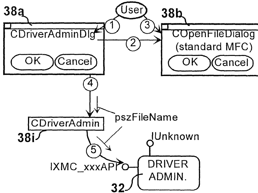
FIG. 55 Scenario-Map - Adding a Driver
