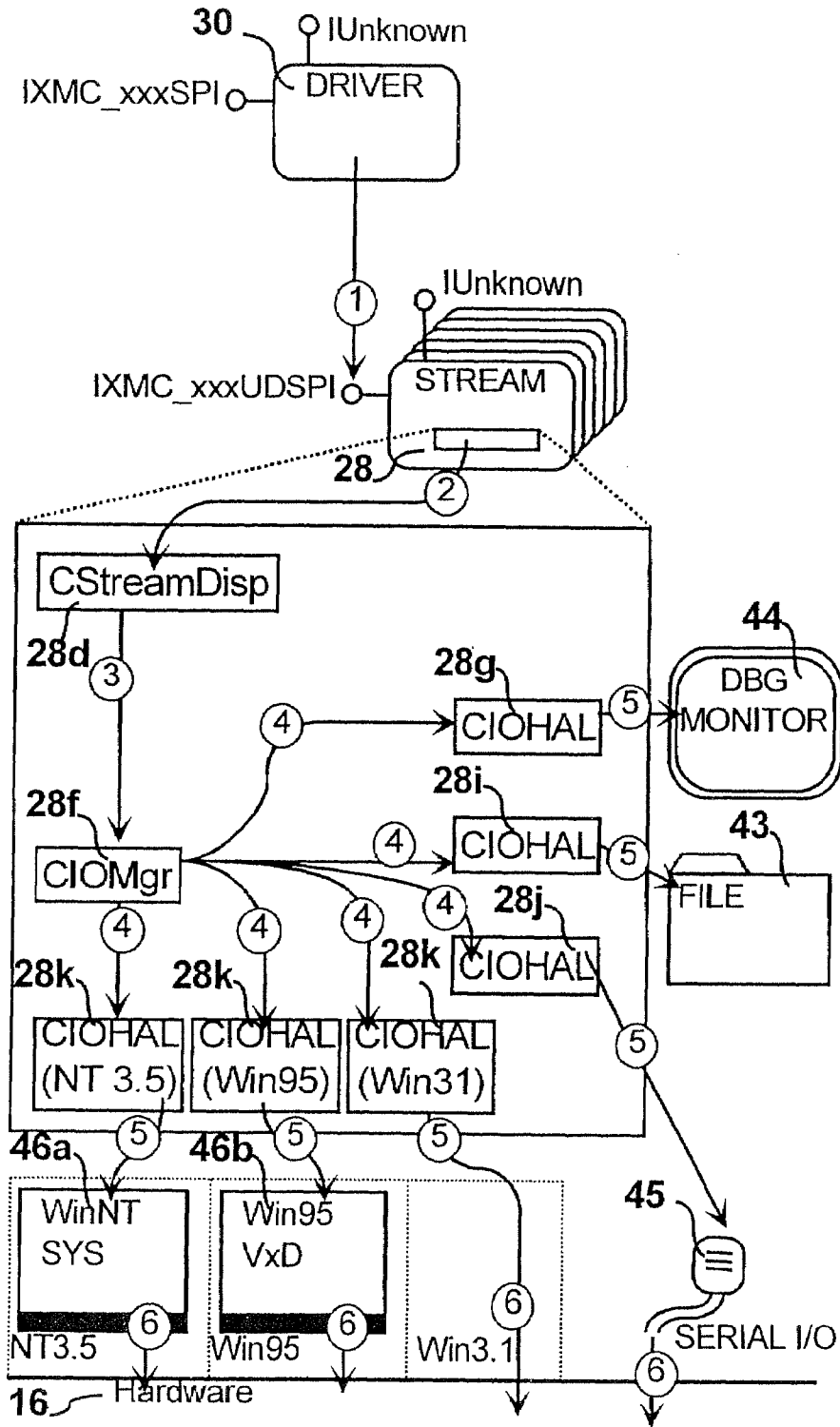
FIG. 29 Scenario-Map - Opening the Stream
