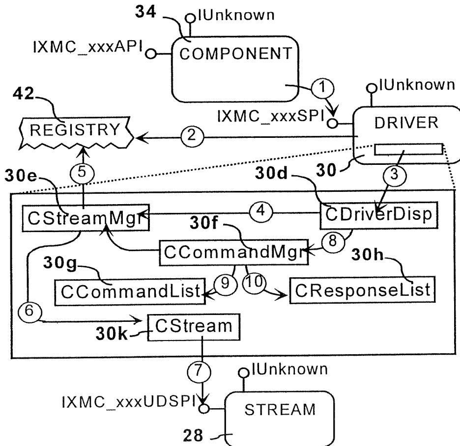
FIG. 18 Scenario-Map - Init. by Component
