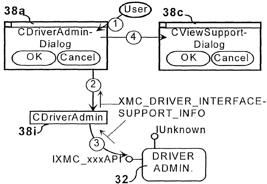
FIG. 57 Scenario-Map - View Support
