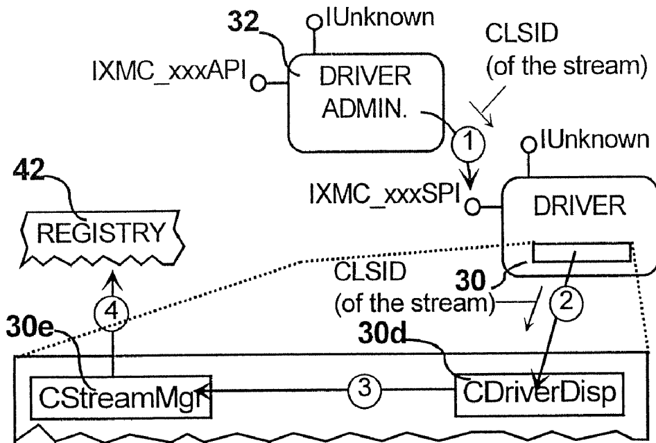
FIG. 16 Scenario-Map - Query Operation
