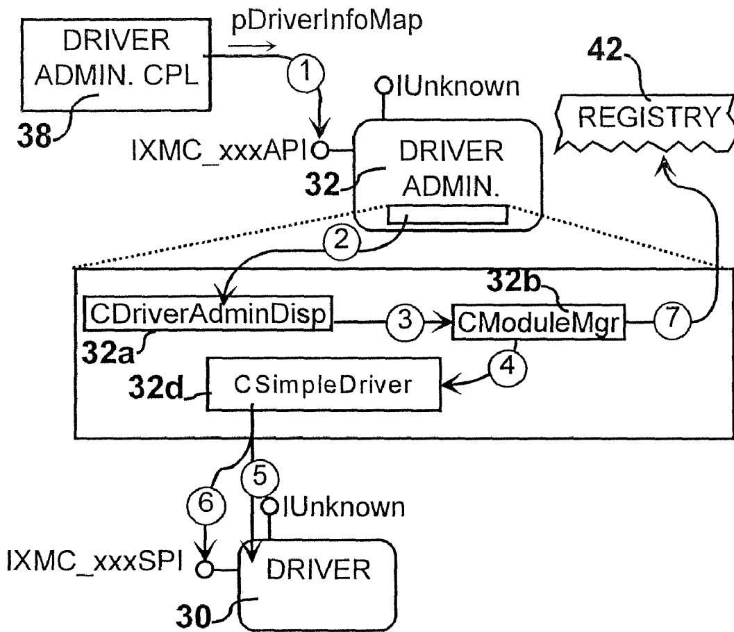
FIG. 43 Scenario-Map - Registering a Driver
