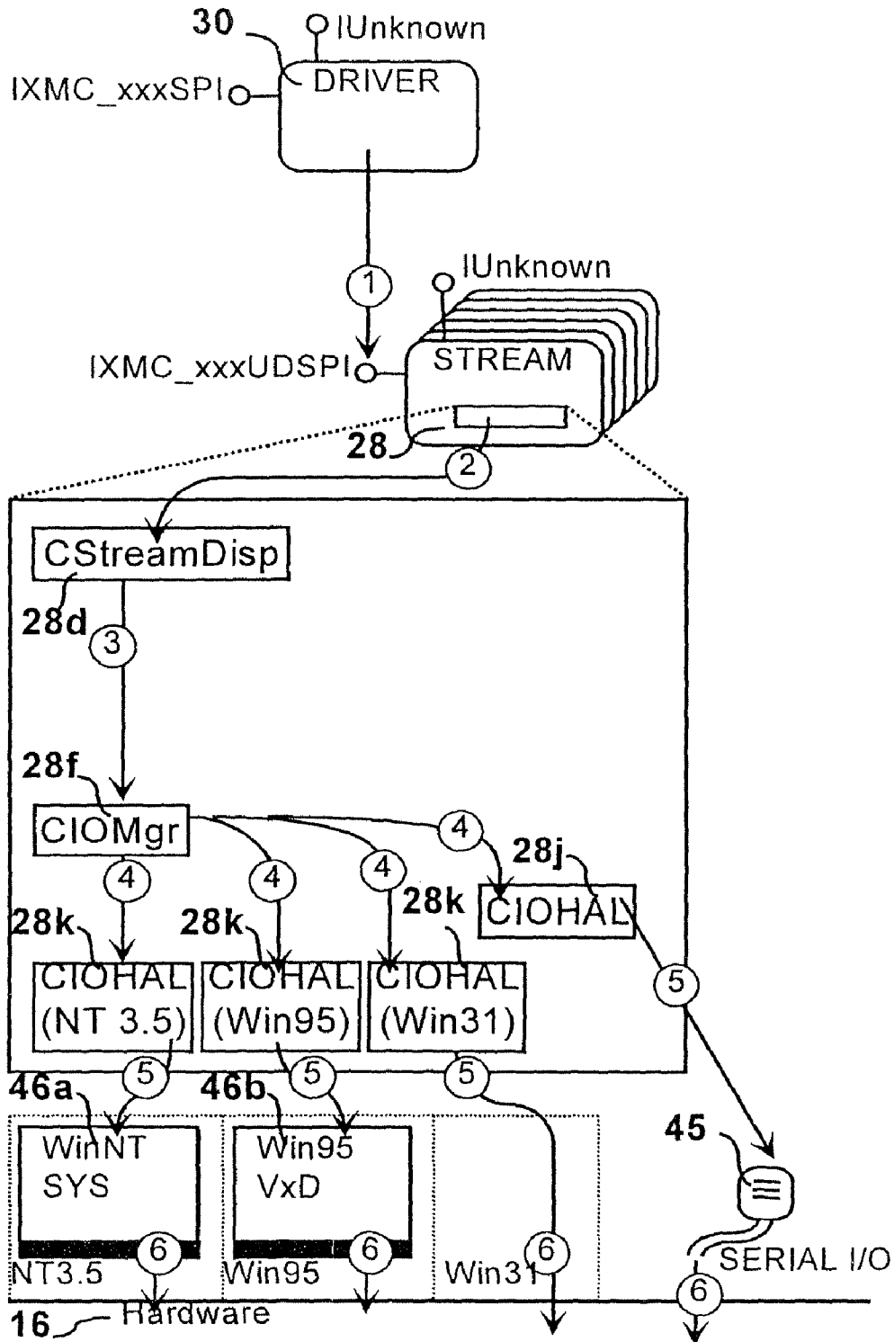
FIG. 31 Scenario-Map - Reading Data
