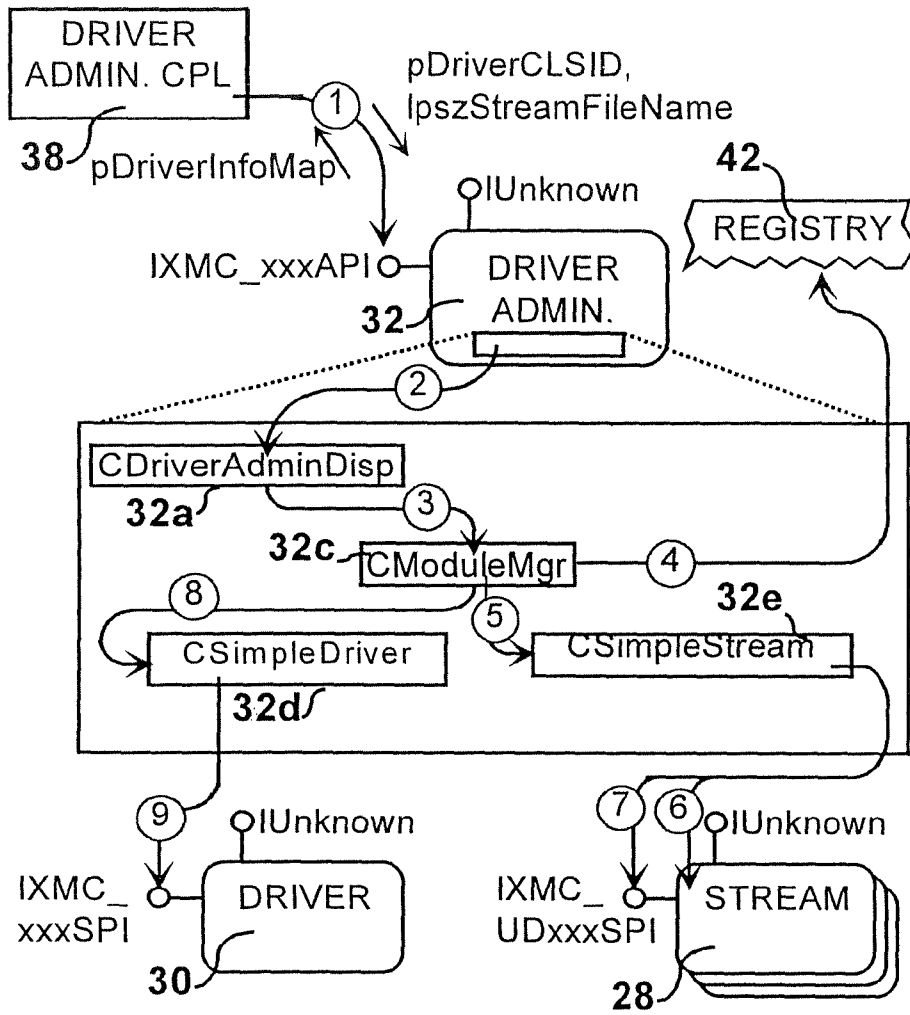
FIG. 44 Scenario-Map - Registering a Stream
