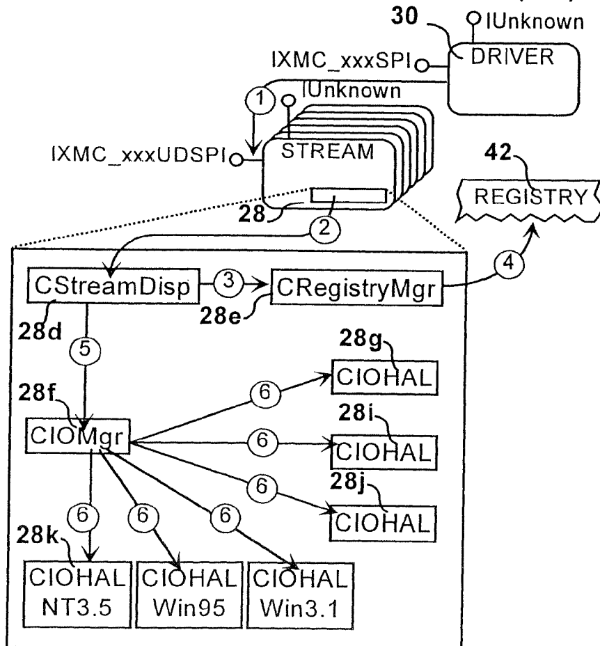
FIG. 28 Scenario-Map - Initialization (Drv)
