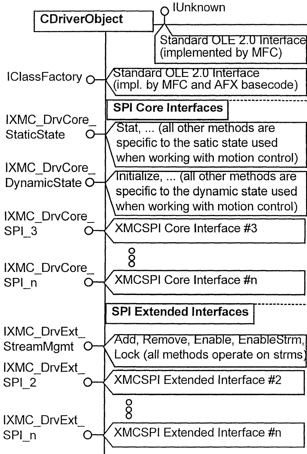
FIG. 21 Interface-Map
