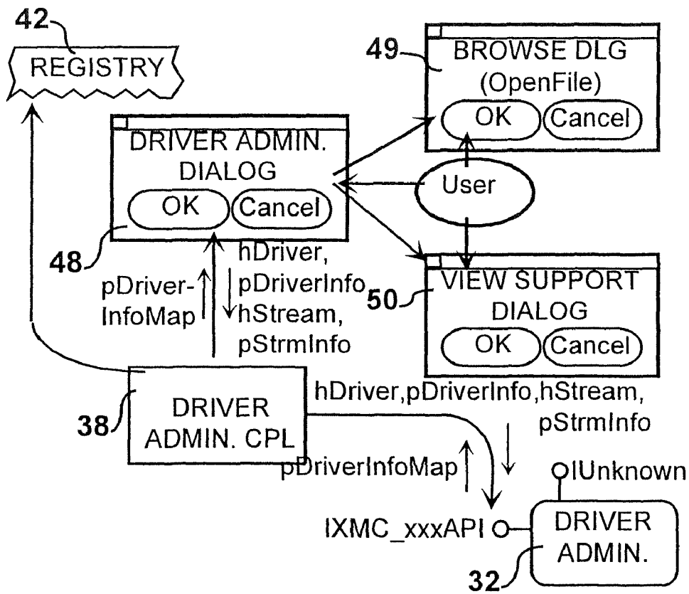
FIG. 51 Module Interaction-Map
