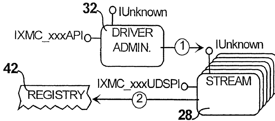
FIG. 25 Scenario-Map - Registration
