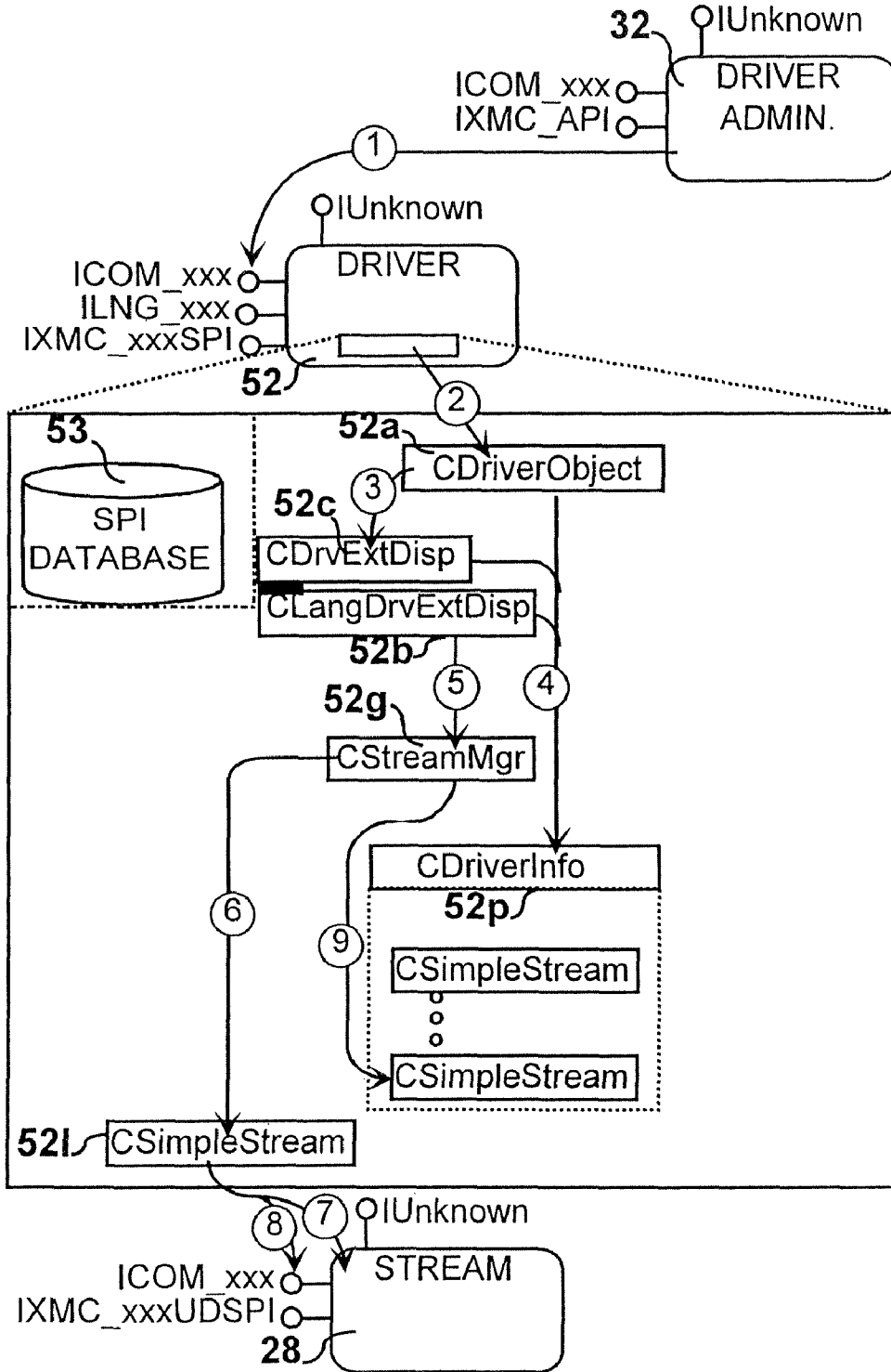
FIG. 61 Scenario-Map - Adding a Stream
