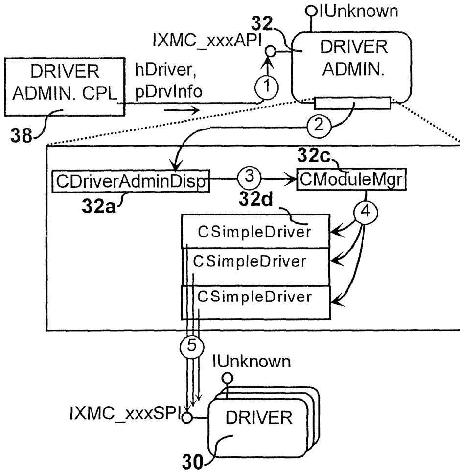
FIG. 45 Scenario-Map - Setting Driver Info.
