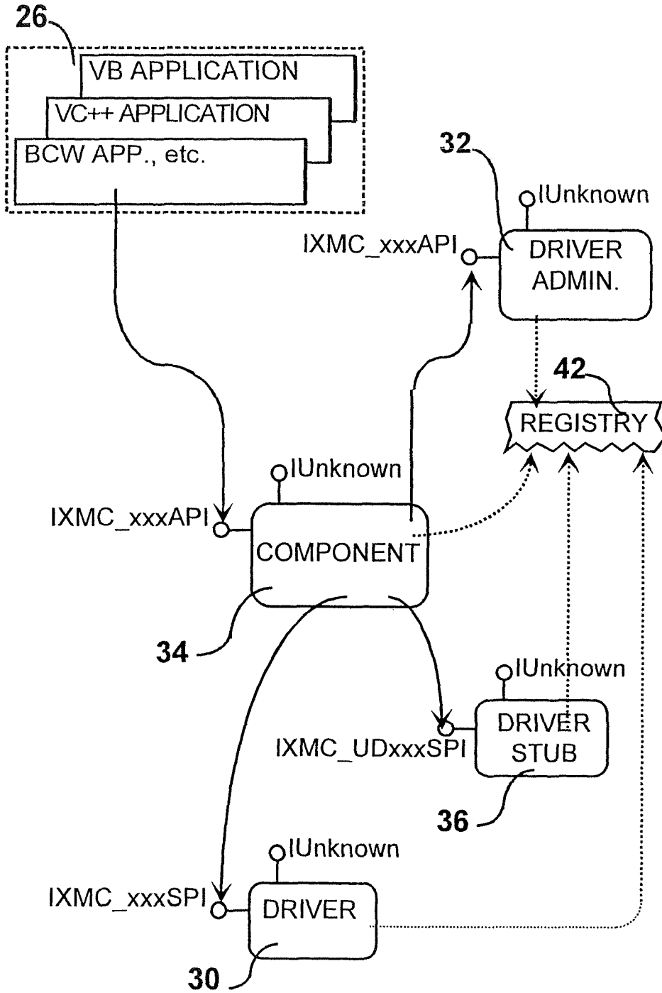
FIG. 2 Module Interaction-Map
