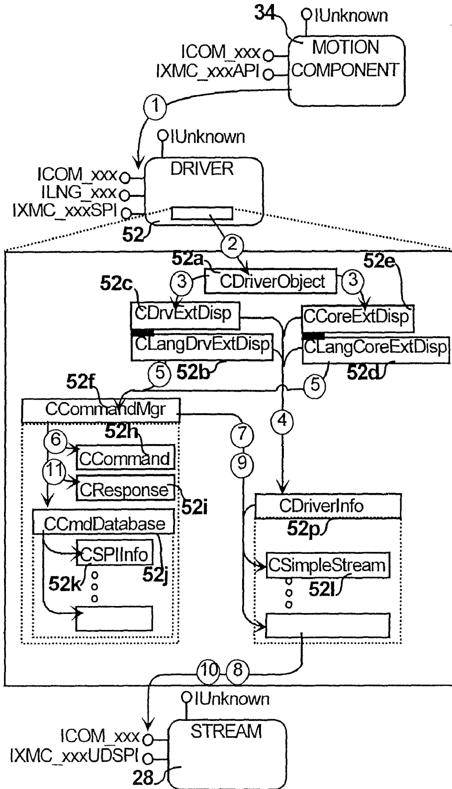
FIG. 65 Scenario-Map - Command Operation
