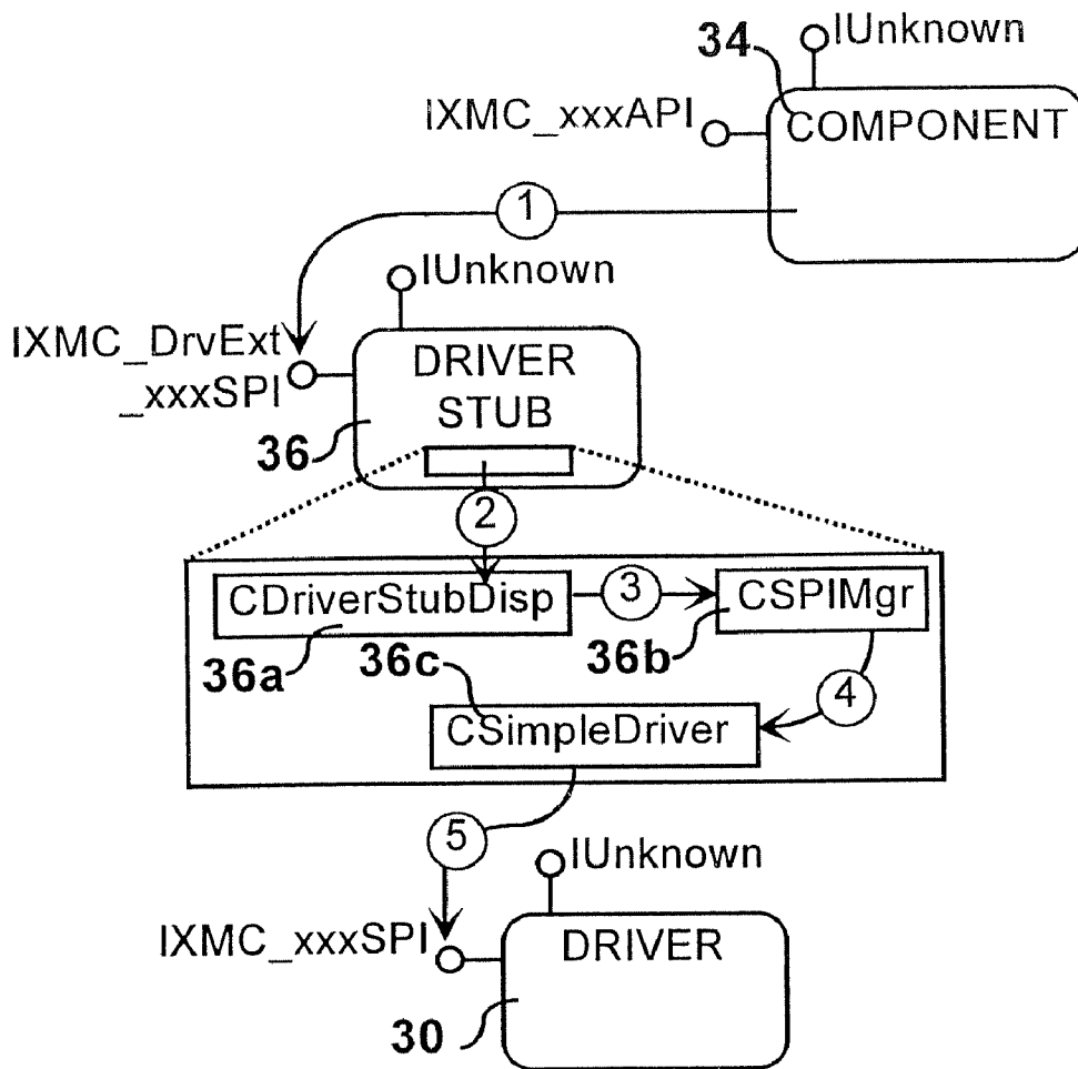
FIG. 37 Scenario-Map - Operations
