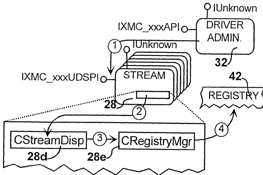
FIG. 27 Scenario-Map - Clean-up
