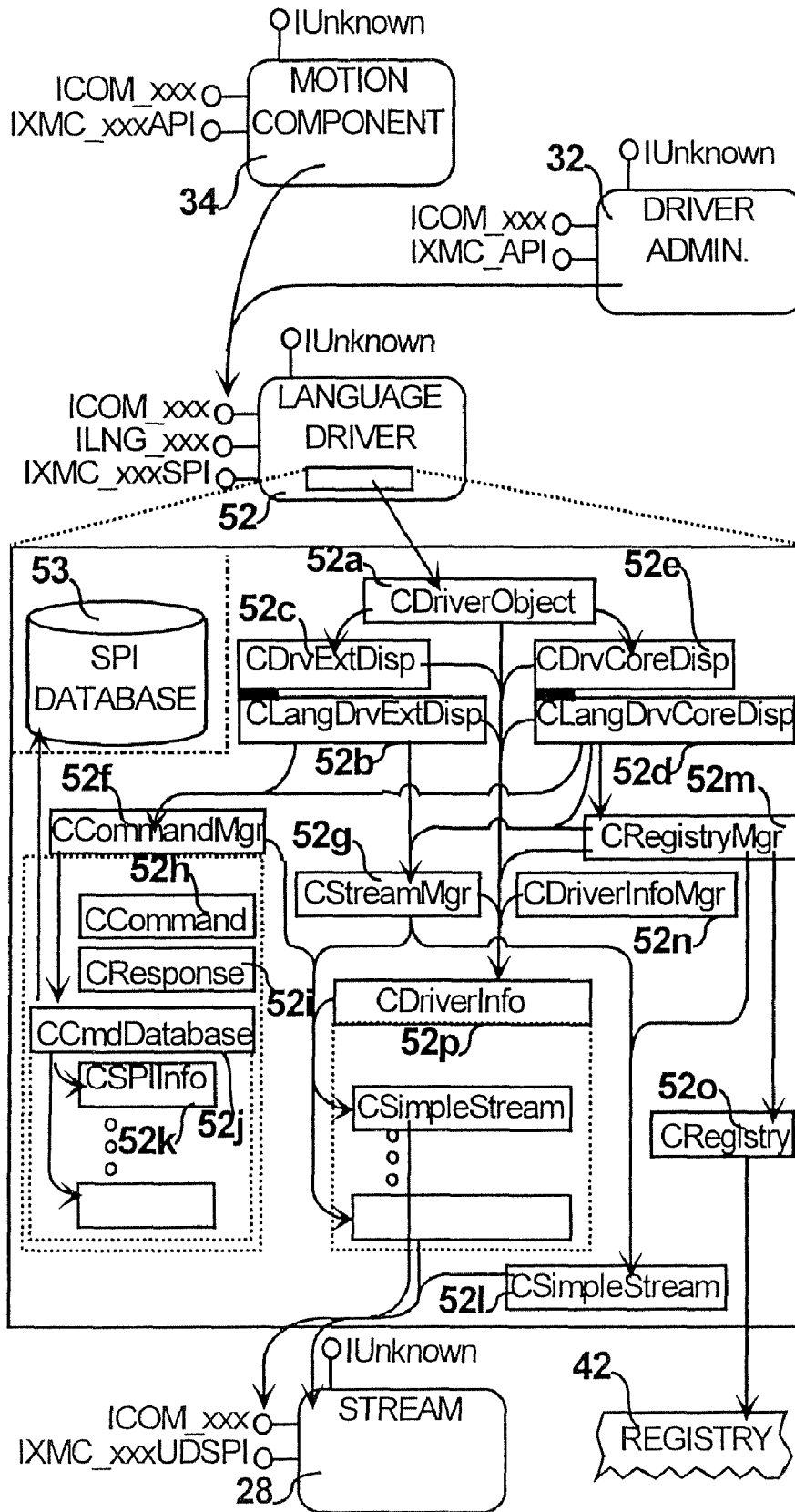
FIG. 59 Object Interaction-Map
