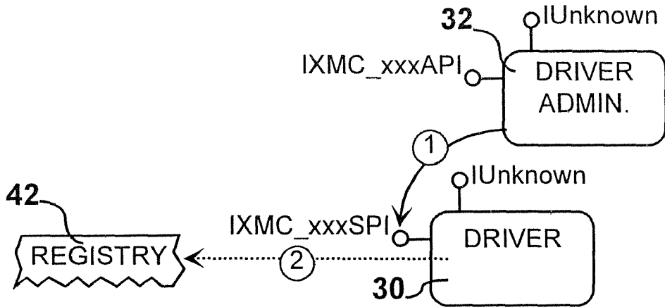
FIG. 13 Scenario-Map - Registration
