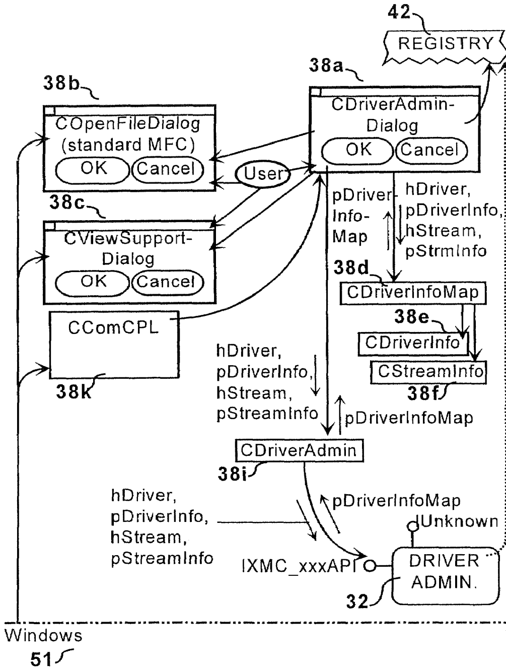
FIG. 52 Object Interaction-Map
