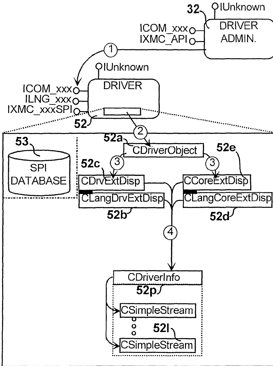
FIG. 62 Scenario-Map - Query Operation
