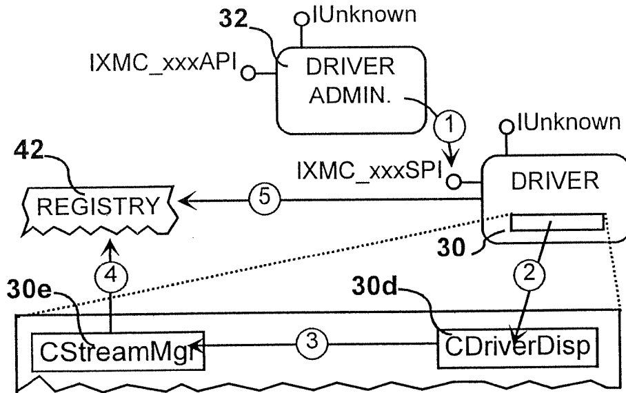
FIG. 17 Scenario-Map - Clean-Up by Drv. Admin.
