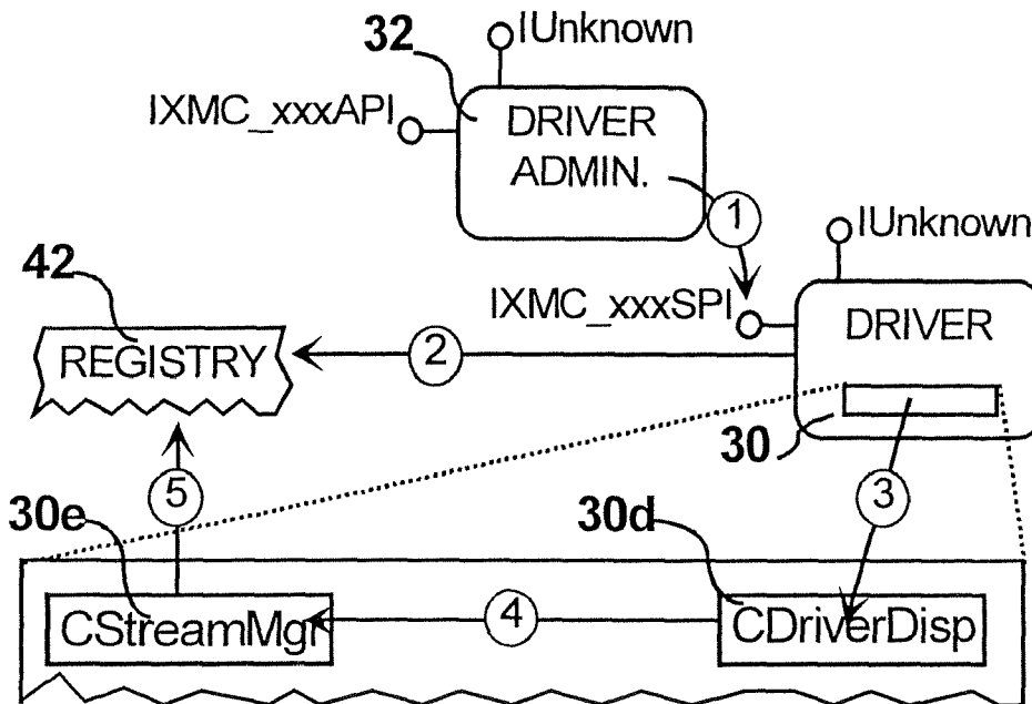
FIG. 14 Scenario-Map - Init. by Driver Admin.
