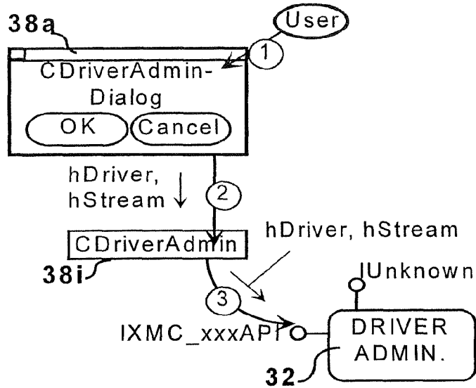
FIG. 56 Scenario-Map - Removing a Driver
