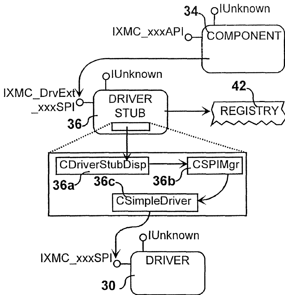
FIG. 35 Object Interaction-Map
