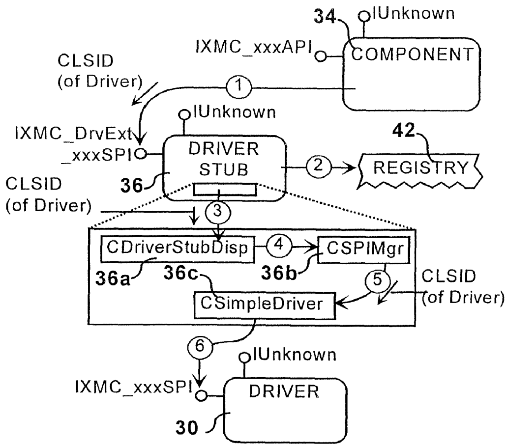
FIG. 36 Scenario-Map - Initialization
