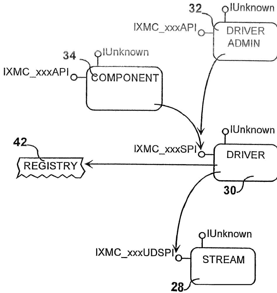
FIG. 11 Module Interaction-Map
