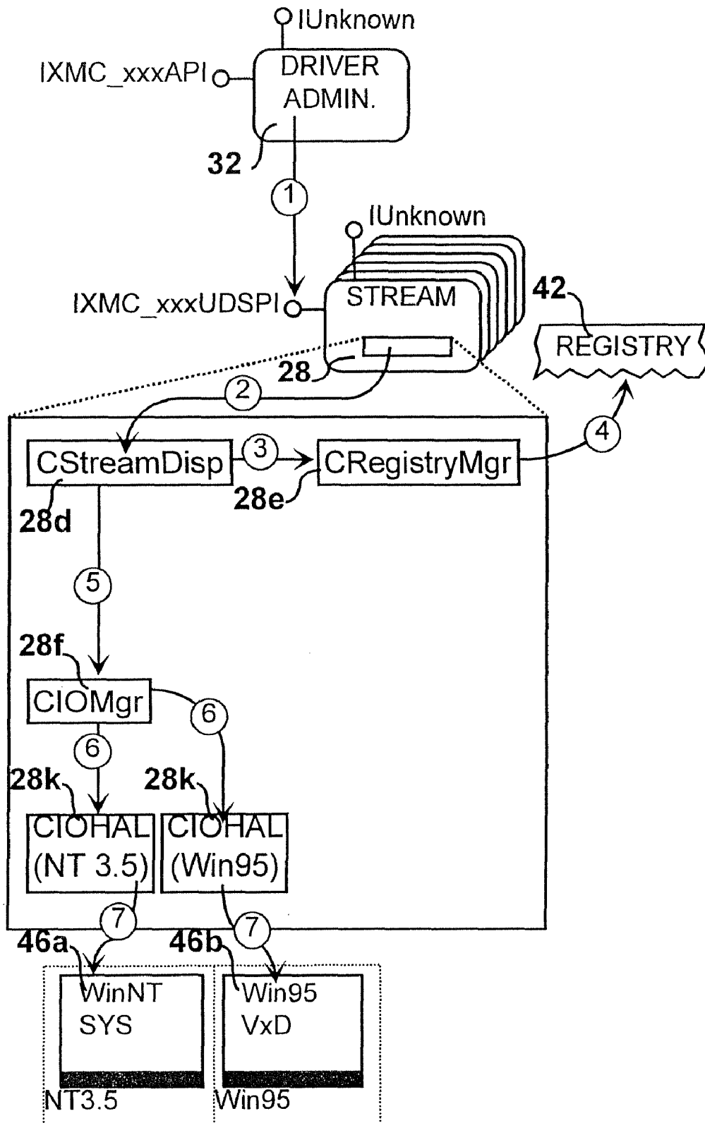
FIG. 24 Scenario-Map - Initialization
