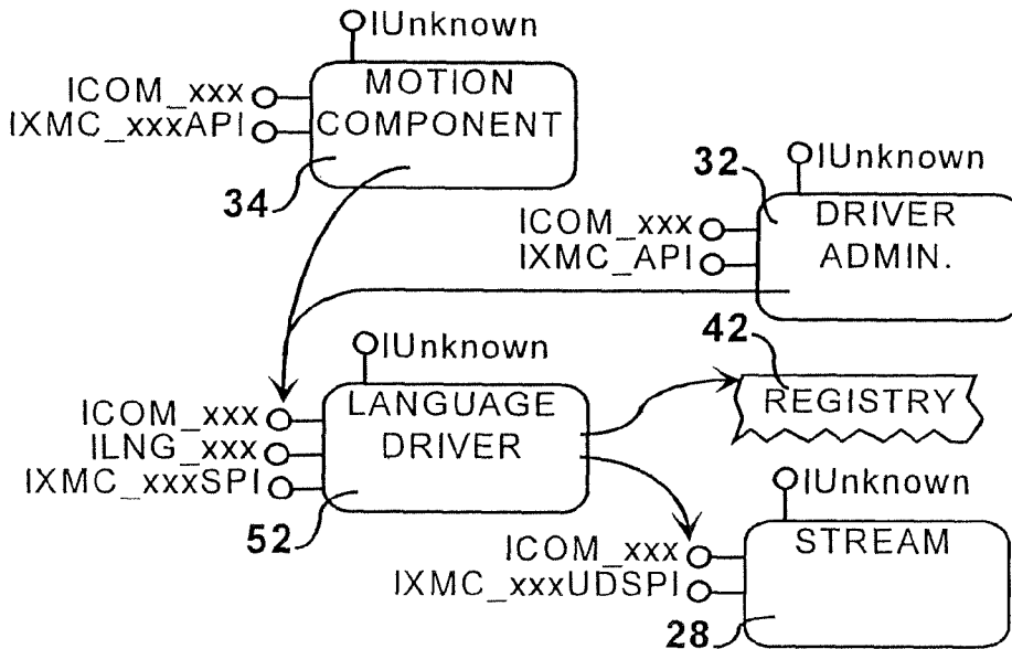
FIG. 58 Module Interaction-Map
