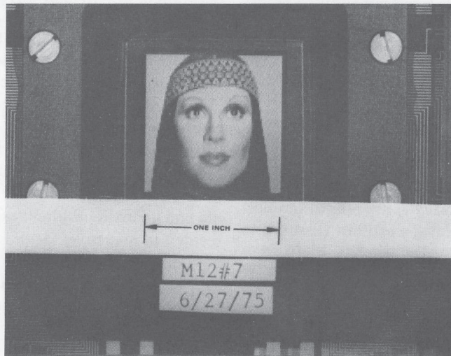
Fig. 11-18. Silicon Extrinsic Matrix: An array of transistors is fabricated on a single-crystal silicon wafer. The circuitry is similar to the TFT design with the liquid crystal in contact with the transistors. Silicon transistor action is much better understood and more reliable than TFT operation, but the substrate is opaque, expensive, and limited in area. An example of a picture displayed on a Hughes array is also shown. (John Gunther)
