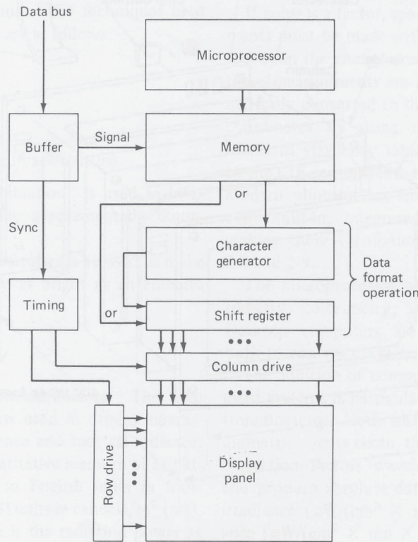
Fig. 2-6. Electronics for control and drive of displays.
