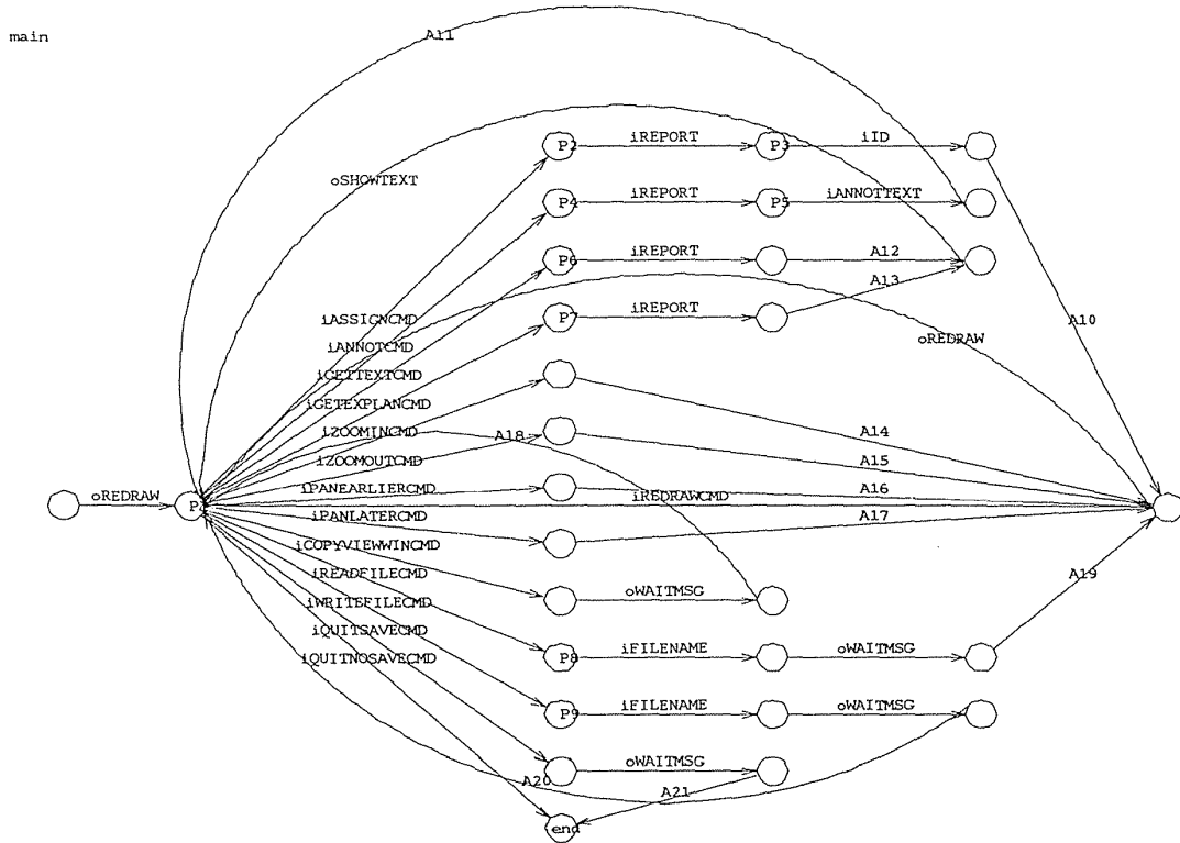
Figure 8.1 Transition diagram indicating user inputs with an "i" and computer outputs with an "o." This relatively simple diagram shows only a portion of the system. Complete transition diagrams may comprise many pages. (Courtesy of Robert J. K. Jacob, Naval Research Laboratory, Washington, D.C.)
