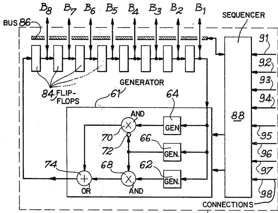
FIG. 5 GENERATOR 26 (26')
