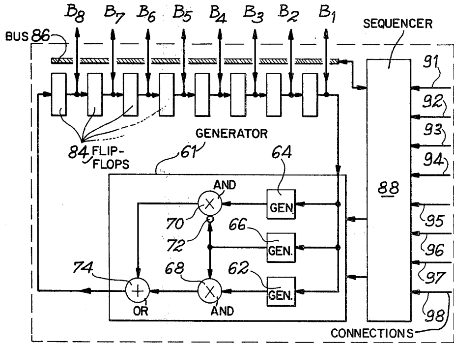
FIG. 5 GENERATOR 26 (26')
