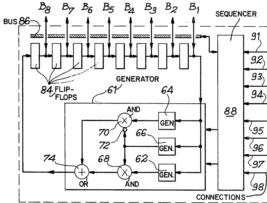
FIG. 5 GENERATOR 26 (26')
