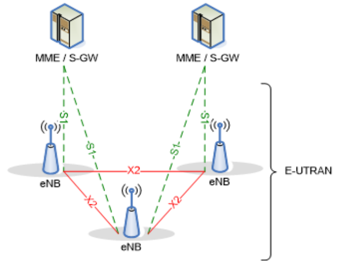
Figure 4-1: Overall Architecture
