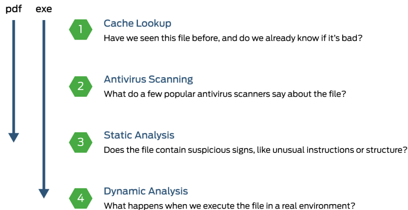
Figure 1: Example Sky ATP Pipeline Approach for Analyzing Malware
