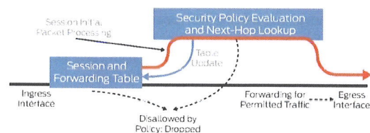
Figure 3: Session-based forwarding algorithm
