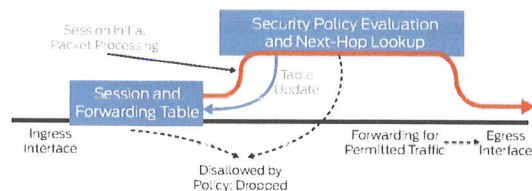
Figure 3: Session-based forwarding algorithm
