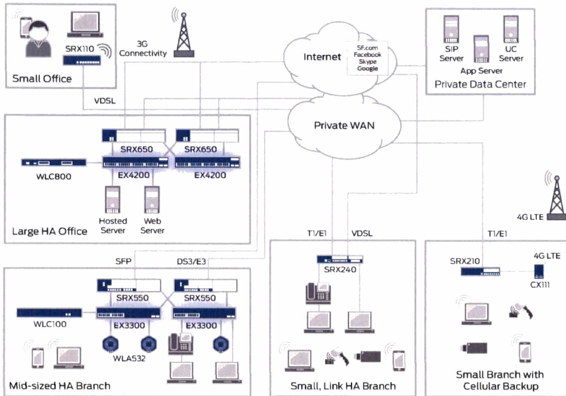
Figure 4 The distributed enterprise
