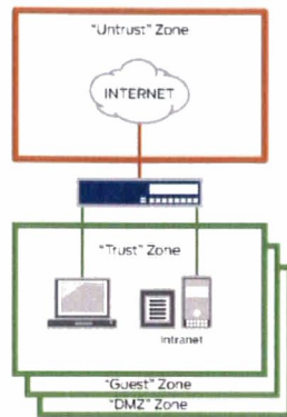
Figure 1: Firewalls, zones and policies
